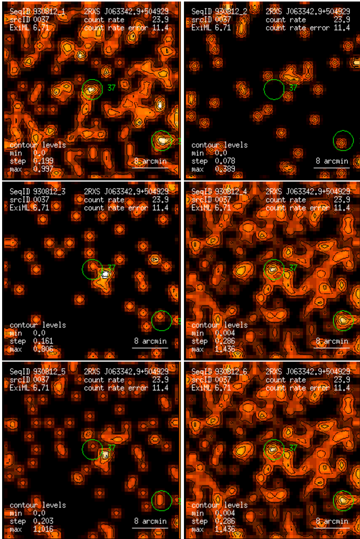
Figure 37: RASS 930812: detection 0037: band rate images, Gaussian filter: (1) PSPC channels 11 – 41, (2) 52 – 90, (3) 91 – 201, (4) 11 – 235, (5) 52 – 201, (6) 11 – 201. Broad band rates in counts/ks. Band rate contour levels in counts/ks/arcmin 2 .
