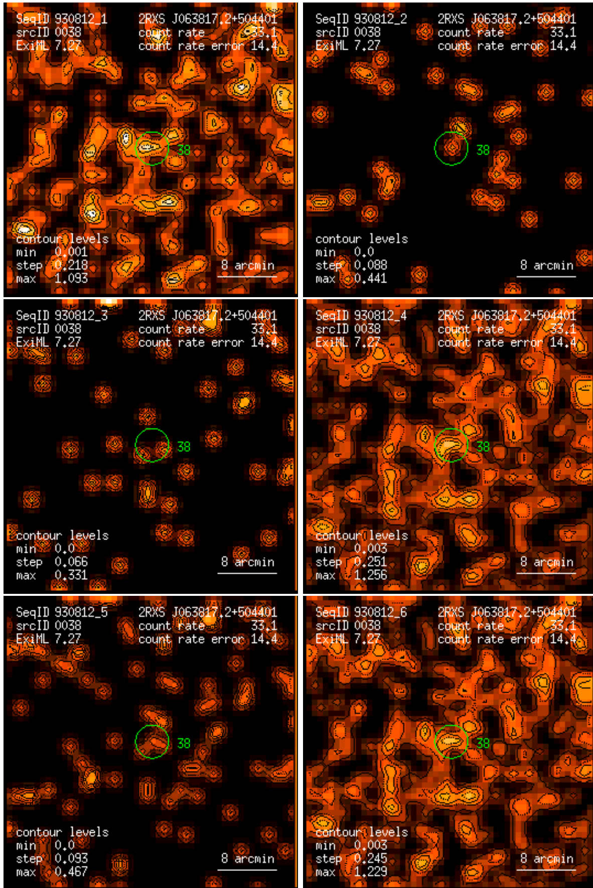
Figure 38: RASS 930812: detection 0038: band rate images, Gaussian filter: (1) PSPC channels 11 – 41, (2) 52 – 90, (3) 91 – 201, (4) 11 – 235, (5) 52 – 201, (6) 11 – 201. Broad band rates in counts/ks. Band rate contour levels in counts/ks/arcmin 2 .
