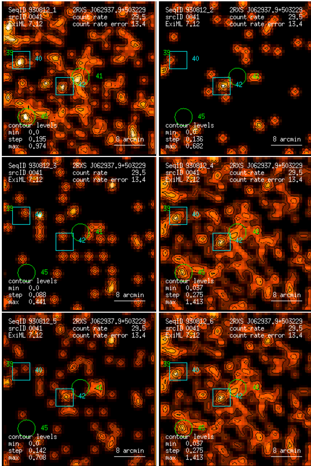
Figure 41: RASS 930812: detection 0041: band rate images, Gaussian filter: (1) PSPC channels 11 – 41, (2) 52 – 90, (3) 91 – 201, (4) 11 – 235, (5) 52 – 201, (6) 11 – 201. Broad band rates in counts/ks. Band rate contour levels in counts/ks/arcmin 2 .
