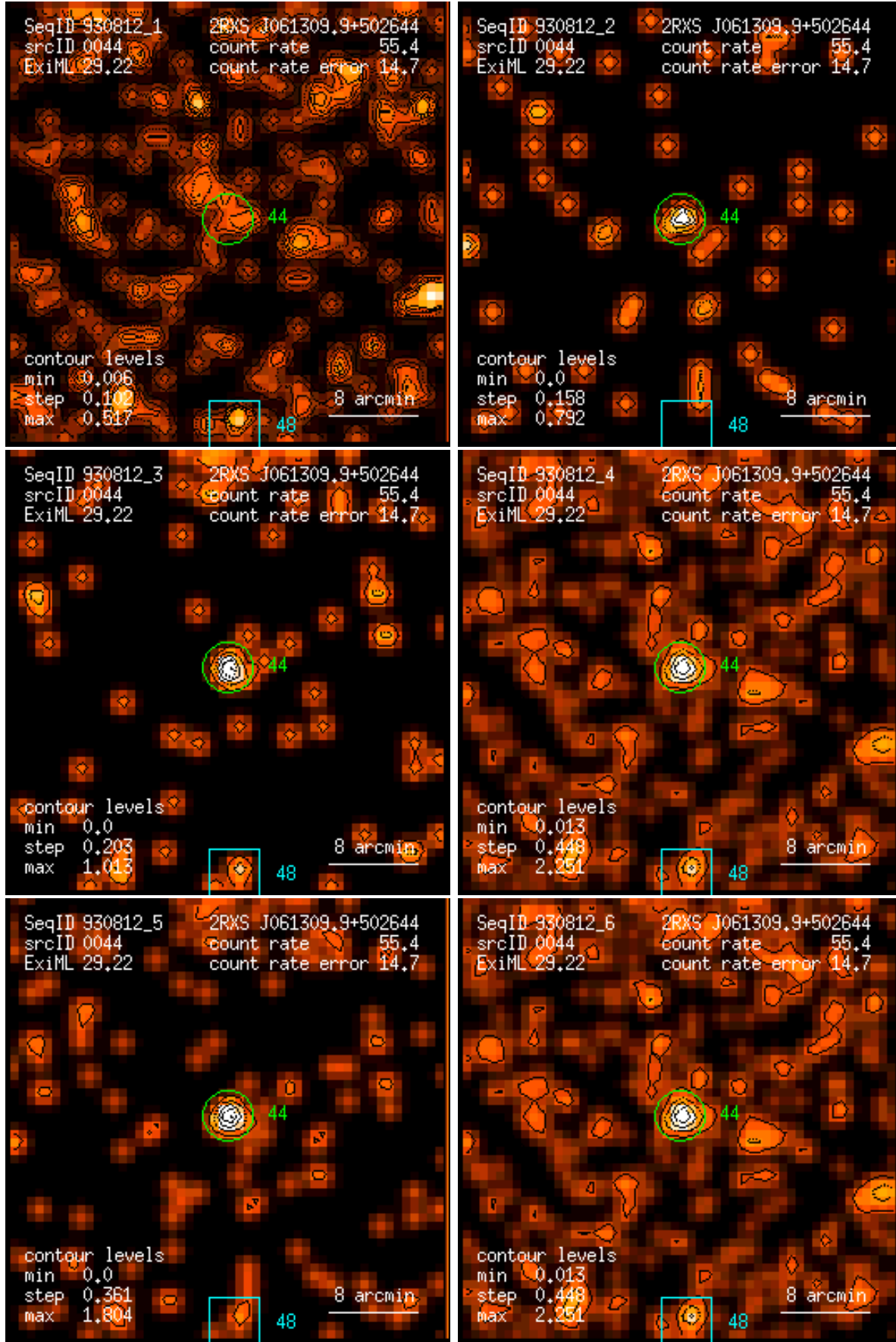
Figure 44: RASS 930812: detection 0044: band rate images, Gaussian filter: (1) PSPC channels 11 – 41, (2) 52 – 90, (3) 91 – 201, (4) 11 – 235, (5) 52 – 201, (6) 11 – 201. Broad band rates in counts/ks. Band rate contour levels in counts/ks/arcmin 2 .
