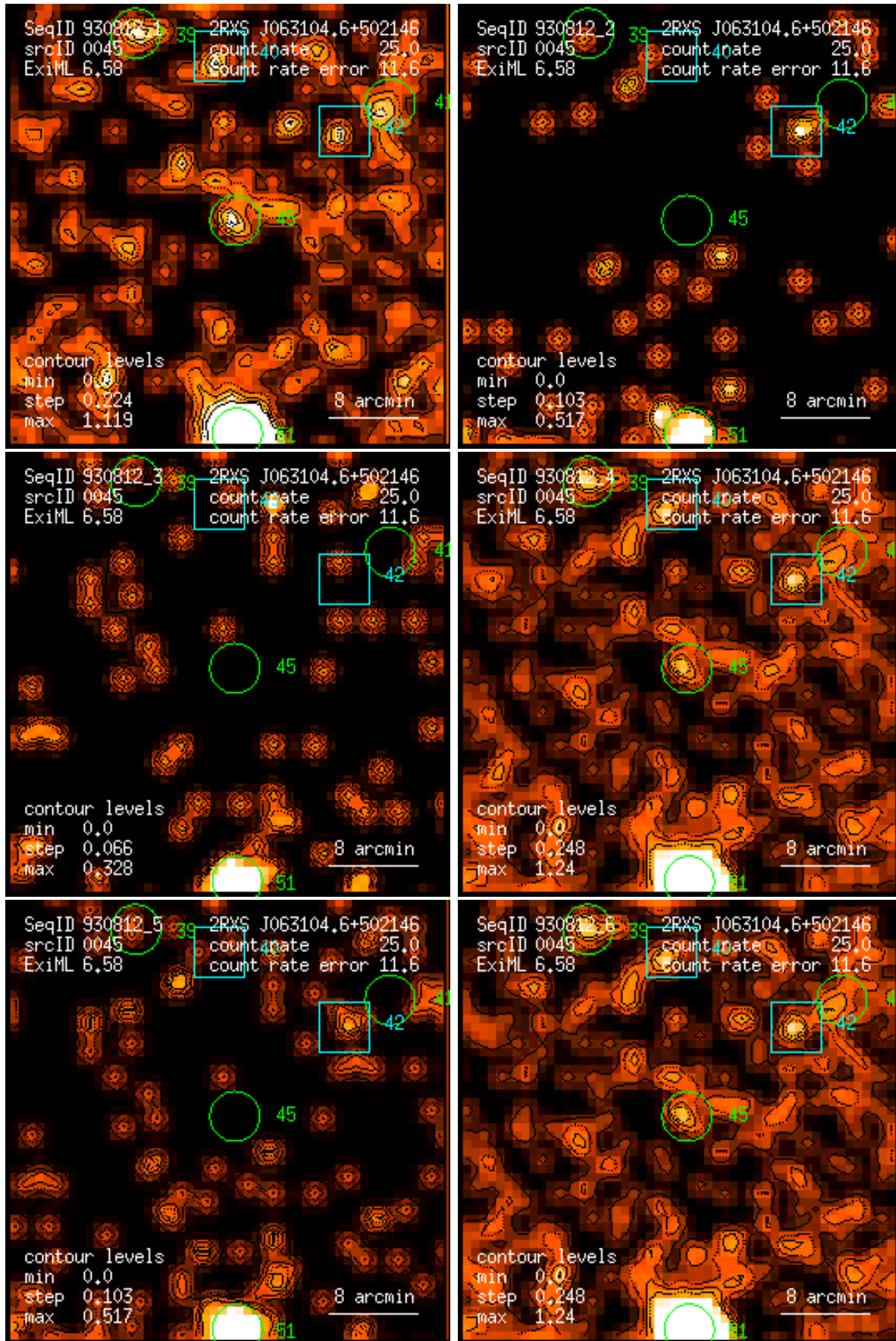
Figure 45: RASS 930812: detection 0045: band rate images, Gaussian filter: (1) PSPC channels 11 – 41, (2) 52 – 90, (3) 91 – 201, (4) 11 – 235, (5) 52 – 201, (6) 11 – 201. Broad band rates in counts/ks. Band rate contour levels in counts/ks/arcmin 2 .
