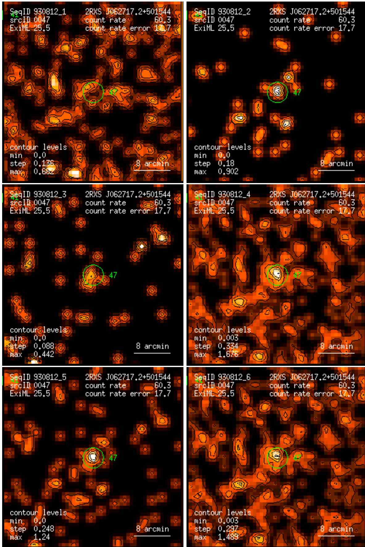
Figure 47: RASS 930812: detection 0047: band rate images, Gaussian filter: (1) PSPC channels 11 – 41, (2) 52 – 90, (3) 91 – 201, (4) 11 – 235, (5) 52 – 201, (6) 11 – 201. Broad band rates in counts/ks. Band rate contour levels in counts/ks/arcmin 2 .
