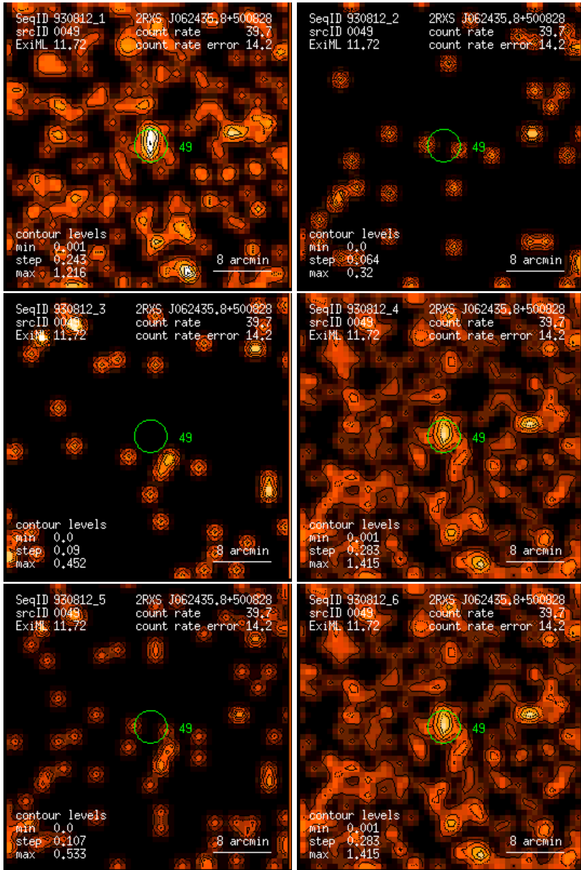
Figure 49: RASS 930812: detection 0049: band rate images, Gaussian filter: (1) PSPC channels 11 – 41, (2) 52 – 90, (3) 91 – 201, (4) 11 – 235, (5) 52 – 201, (6) 11 – 201. Broad band rates in counts/ks. Band rate contour levels in counts/ks/arcmin 2 .
