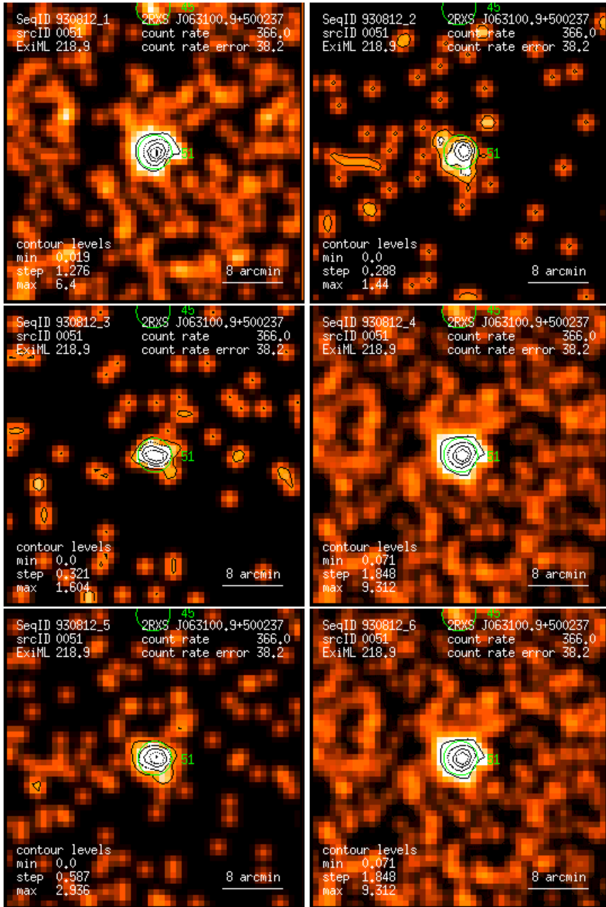
Figure 51: RASS 930812: detection 0051: band rate images, Gaussian filter: (1) PSPC channels 11 – 41, (2) 52 – 90, (3) 91 – 201, (4) 11 – 235, (5) 52 – 201, (6) 11 – 201. Broad band rates in counts/ks. Band rate contour levels in counts/ks/arcmin 2 .
