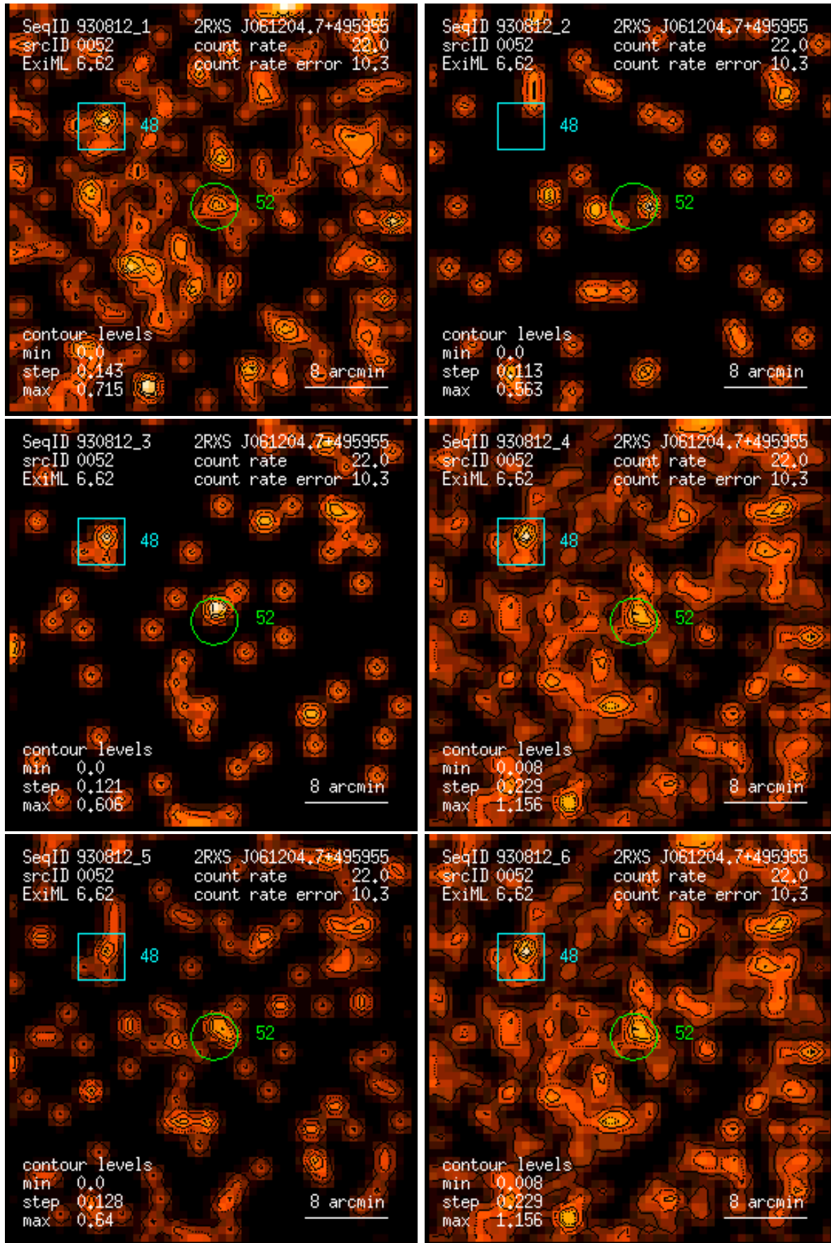
Figure 52: RASS 930812: detection 0052: band rate images, Gaussian filter: (1) PSPC channels 11 – 41, (2) 52 – 90, (3) 91 – 201, (4) 11 – 235, (5) 52 – 201, (6) 11 – 201. Broad band rates in counts/ks. Band rate contour levels in counts/ks/arcmin 2 .
