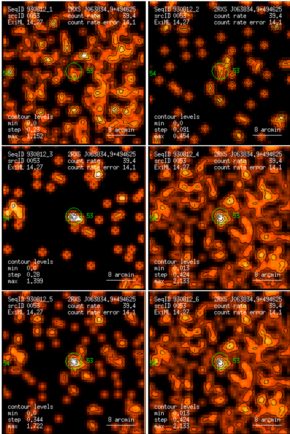
Figure 53: RASS 930812: detection 0053: band rate images, Gaussian filter: (1) PSPC channels 11 – 41, (2) 52 – 90, (3) 91 – 201, (4) 11 – 235, (5) 52 – 201, (6) 11 – 201. Broad band rates in counts/ks. Band rate contour levels in counts/ks/arcmin 2 .
