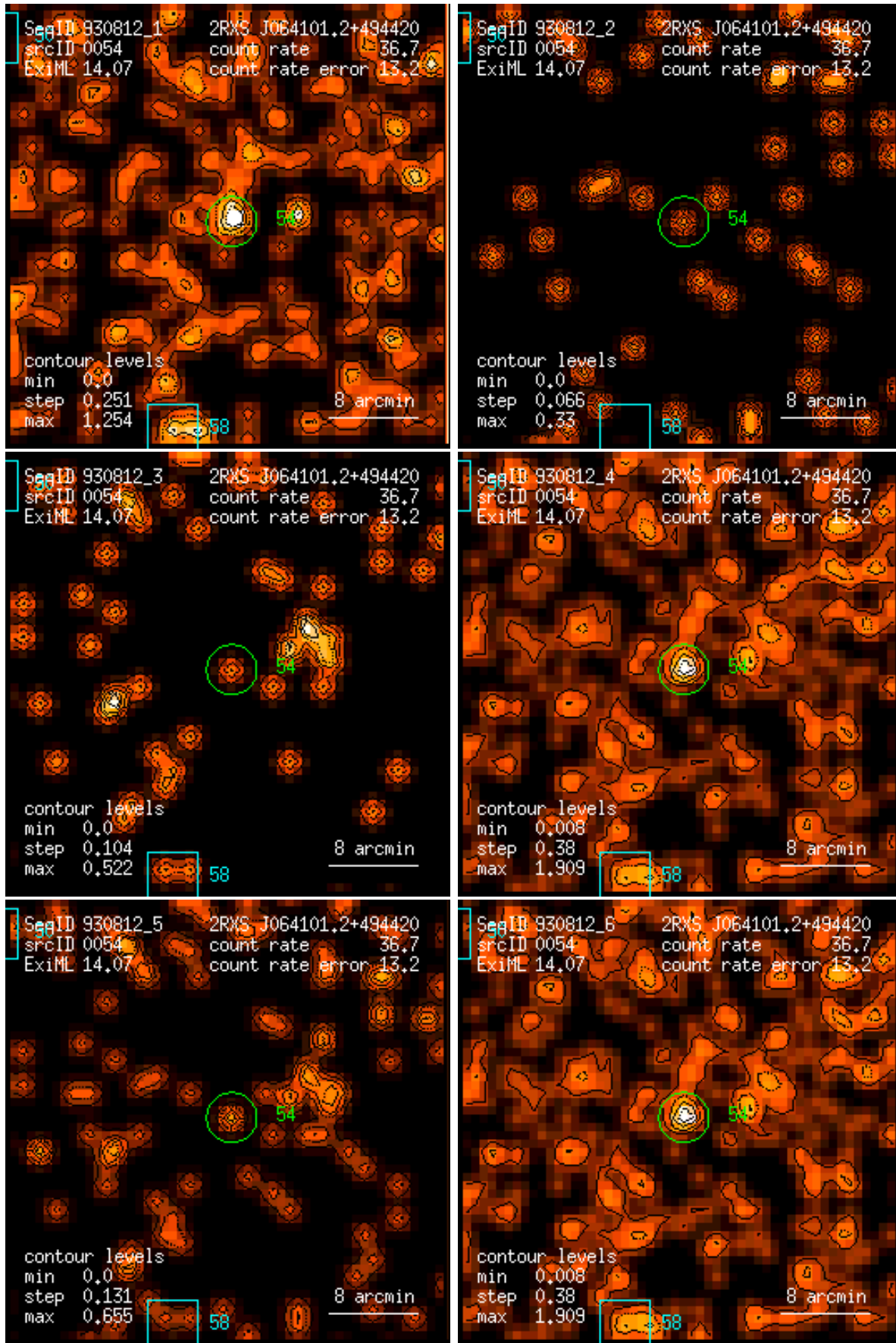
Figure 54: RASS 930812: detection 0054: band rate images, Gaussian filter: (1) PSPC channels 11 – 41, (2) 52 – 90, (3) 91 – 201, (4) 11 – 235, (5) 52 – 201, (6) 11 – 201. Broad band rates in counts/ks. Band rate contour levels in counts/ks/arcmin 2 .
