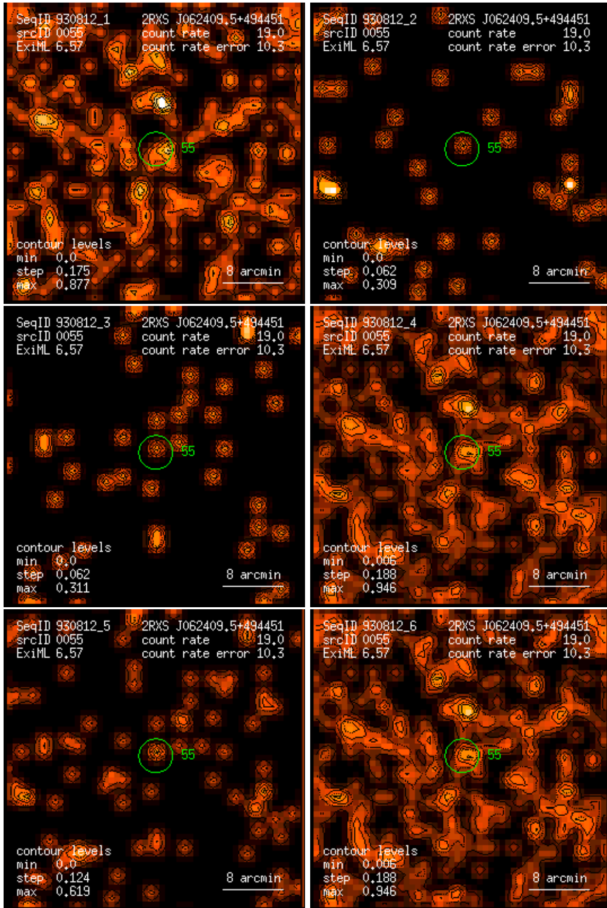
Figure 55: RASS 930812: detection 0055: band rate images, Gaussian filter: (1) PSPC channels 11 – 41, (2) 52 – 90, (3) 91 – 201, (4) 11 – 235, (5) 52 – 201, (6) 11 – 201. Broad band rates in counts/ks. Band rate contour levels in counts/ks/arcmin 2 .
