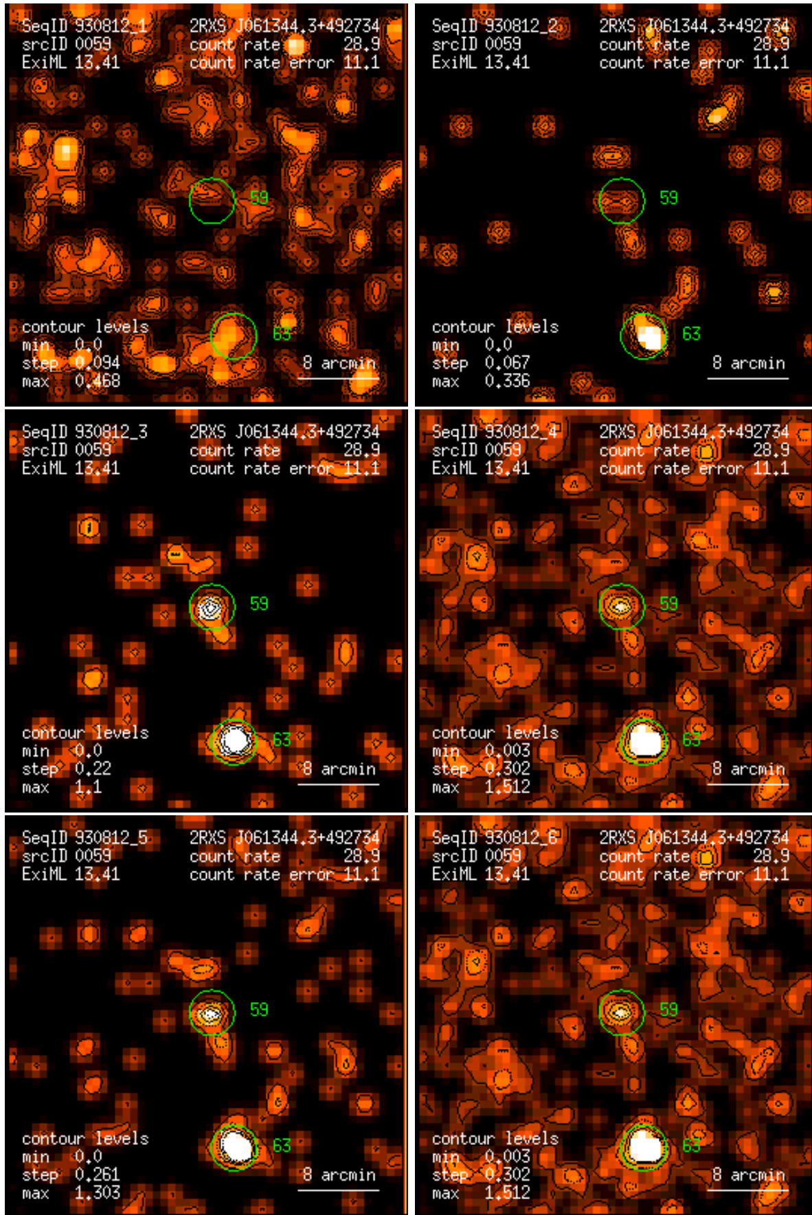
Figure 59: RASS 930812: detection 0059: band rate images, Gaussian filter: (1) PSPC channels 11 – 41, (2) 52 – 90, (3) 91 – 201, (4) 11 – 235, (5) 52 – 201, (6) 11 – 201. Broad band rates in counts/ks. Band rate contour levels in counts/ks/arcmin 2 .
