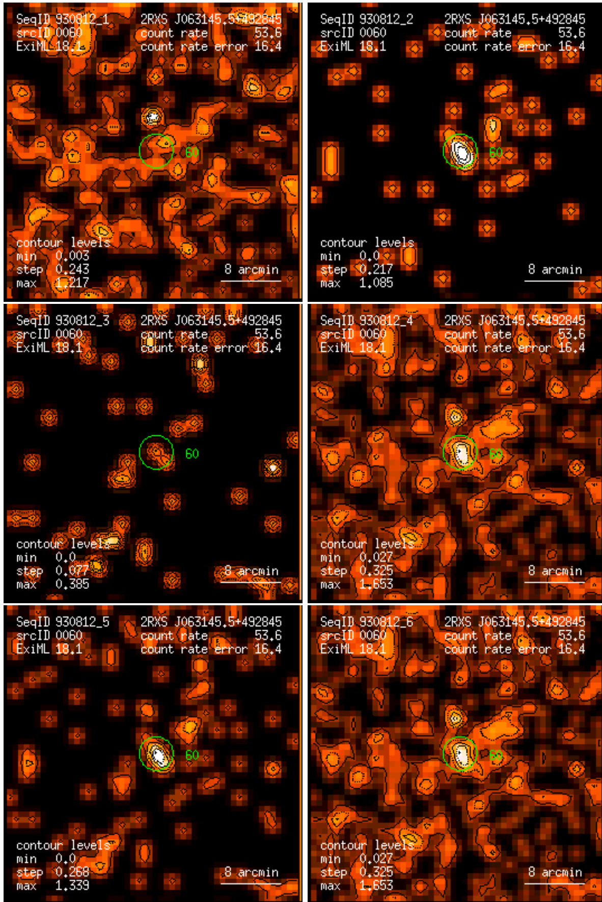
Figure 60: RASS 930812: detection 0060: band rate images, Gaussian filter: (1) PSPC channels 11 – 41, (2) 52 – 90, (3) 91 – 201, (4) 11 – 235, (5) 52 – 201, (6) 11 – 201. Broad band rates in counts/ks. Band rate contour levels in counts/ks/arcmin 2 .
