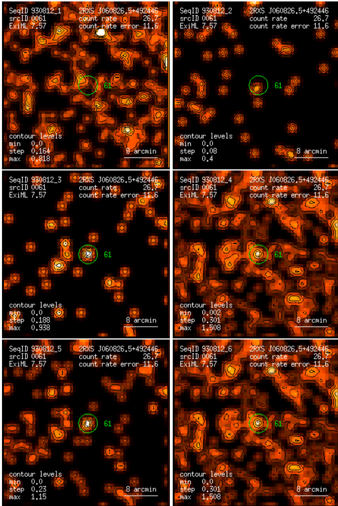
Figure 61: RASS 930812: detection 0061: band rate images, Gaussian filter: (1) PSPC channels 11 – 41, (2) 52 – 90, (3) 91 – 201, (4) 11 – 235, (5) 52 – 201, (6) 11 – 201. Broad band rates in counts/ks. Band rate contour levels in counts/ks/arcmin 2 .
