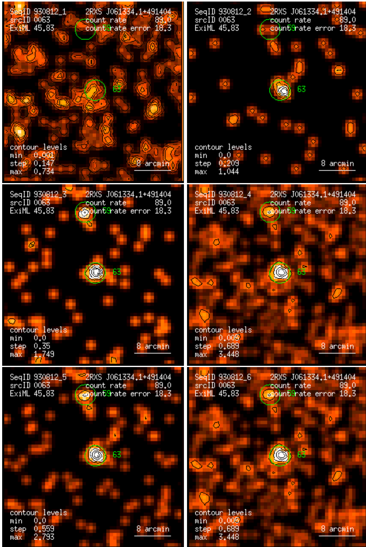
Figure 63: RASS 930812: detection 0063: band rate images, Gaussian filter: (1) PSPC channels 11 – 41, (2) 52 – 90, (3) 91 – 201, (4) 11 – 235, (5) 52 – 201, (6) 11 – 201. Broad band rates in counts/ks. Band rate contour levels in counts/ks/arcmin 2 .
