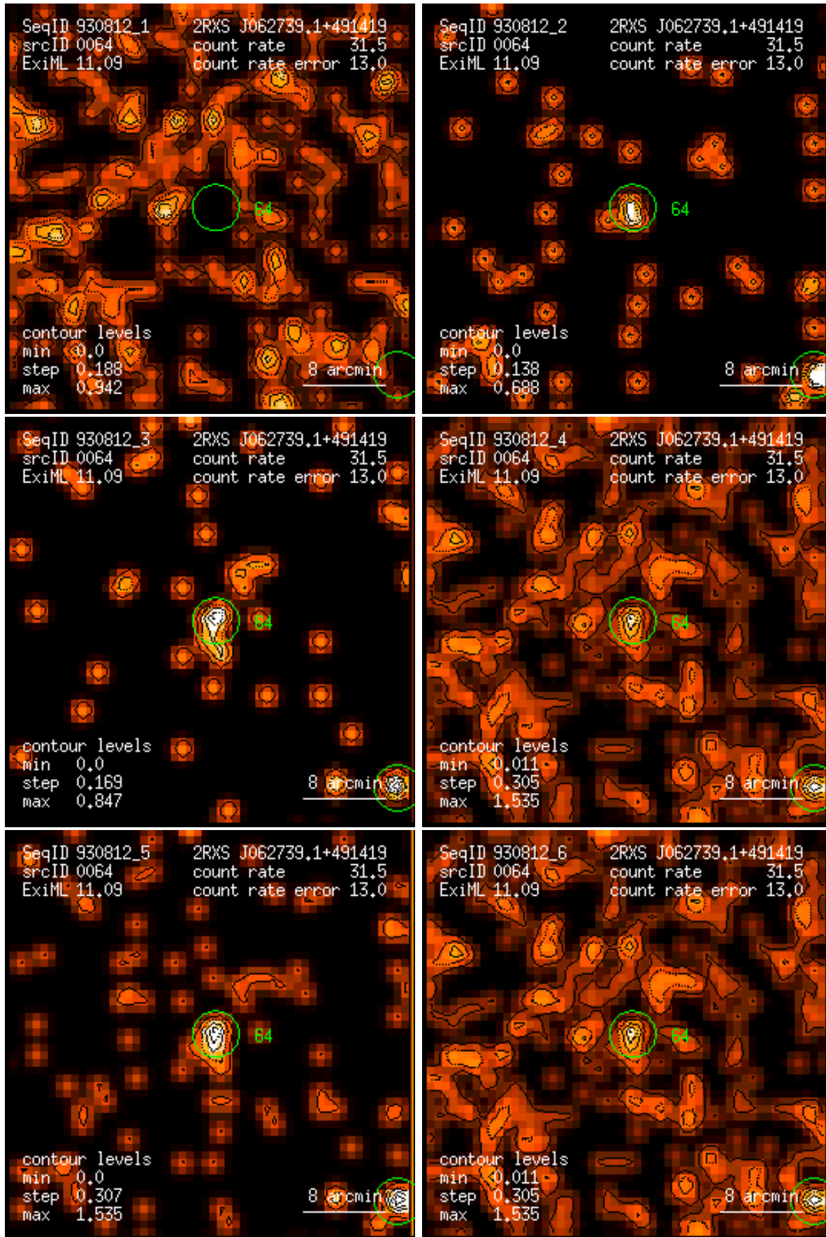
Figure 64: RASS 930812: detection 0064: band rate images, Gaussian filter: (1) PSPC channels 11 – 41, (2) 52 – 90, (3) 91 – 201, (4) 11 – 235, (5) 52 – 201, (6) 11 – 201. Broad band rates in counts/ks. Band rate contour levels in counts/ks/arcmin 2 .
