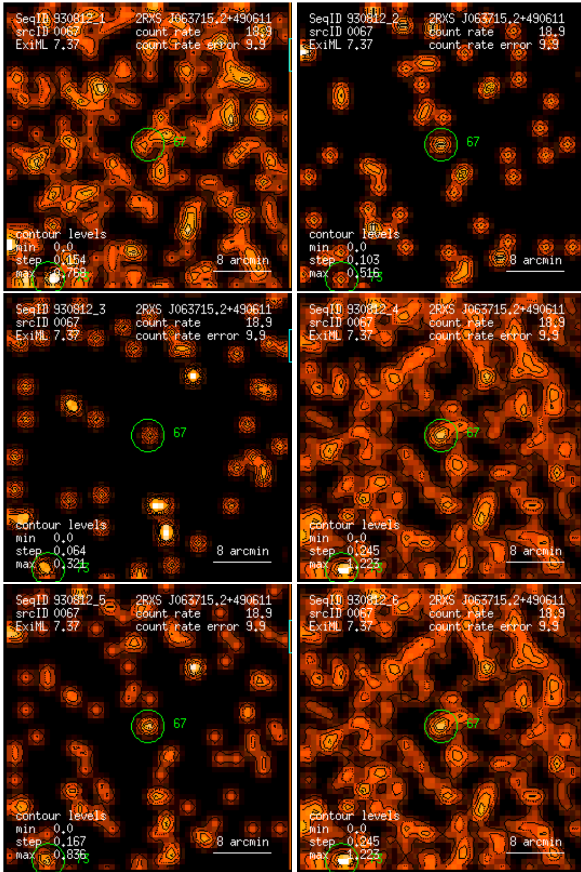
Figure 67: RASS 930812: detection 0067: band rate images, Gaussian filter: (1) PSPC channels 11 – 41, (2) 52 – 90, (3) 91 – 201, (4) 11 – 235, (5) 52 – 201, (6) 11 – 201. Broad band rates in counts/ks. Band rate contour levels in counts/ks/arcmin 2 .
