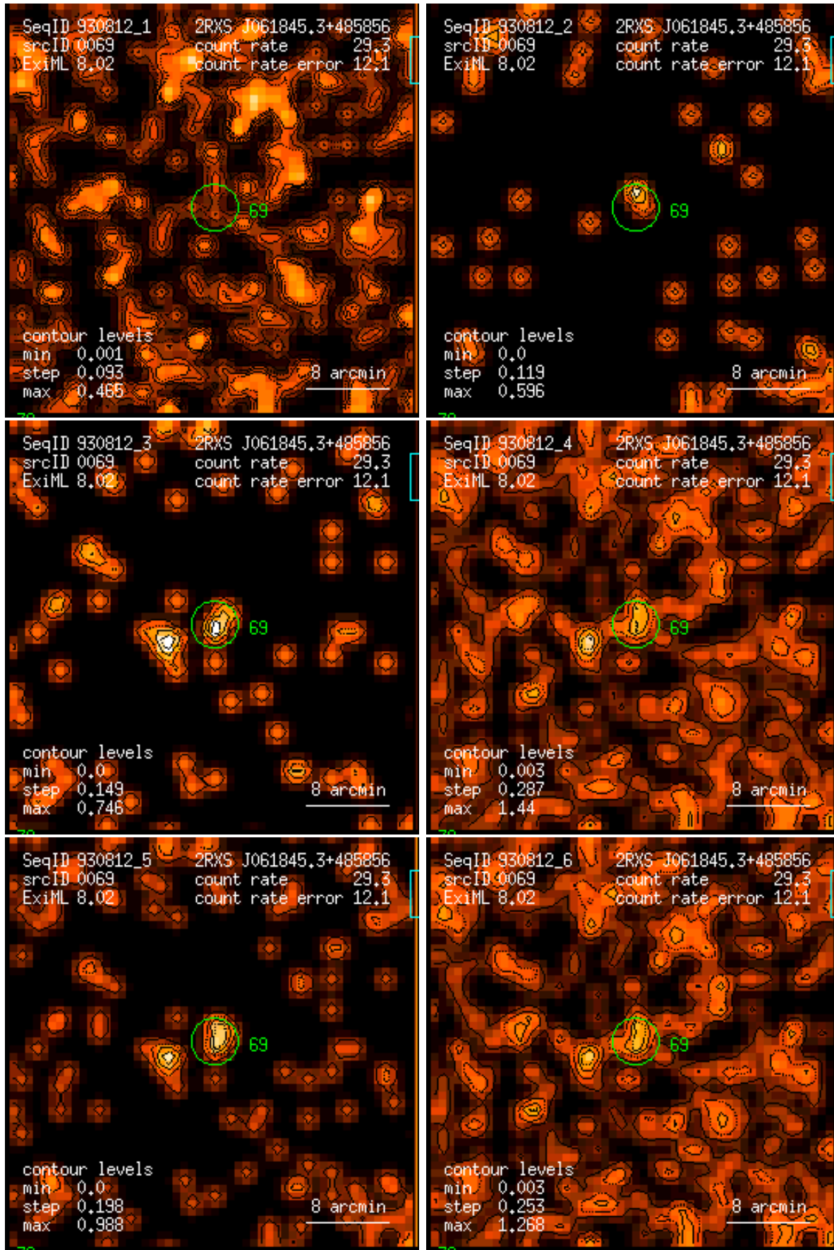
Figure 69: RASS 930812: detection 0069: band rate images, Gaussian filter: (1) PSPC channels 11 – 41, (2) 52 – 90, (3) 91 – 201, (4) 11 – 235, (5) 52 – 201, (6) 11 – 201. Broad band rates in counts/ks. Band rate contour levels in counts/ks/arcmin 2 .
