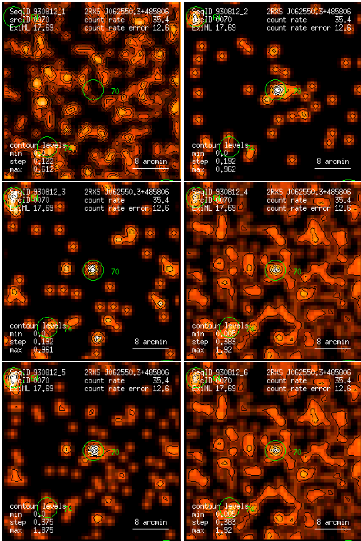
Figure 70: RASS 930812: detection 0070: band rate images, Gaussian filter: (1) PSPC channels 11 – 41, (2) 52 – 90, (3) 91 – 201, (4) 11 – 235, (5) 52 – 201, (6) 11 – 201. Broad band rates in counts/ks. Band rate contour levels in counts/ks/arcmin 2 .
