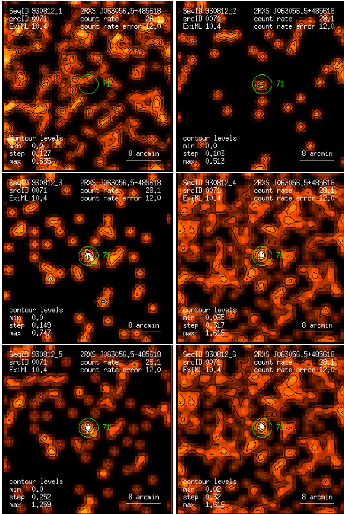
Figure 71: RASS 930812: detection 0071: band rate images, Gaussian filter: (1) PSPC channels 11 – 41, (2) 52 – 90, (3) 91 – 201, (4) 11 – 235, (5) 52 – 201, (6) 11 – 201. Broad band rates in counts/ks. Band rate contour levels in counts/ks/arcmin 2 .
