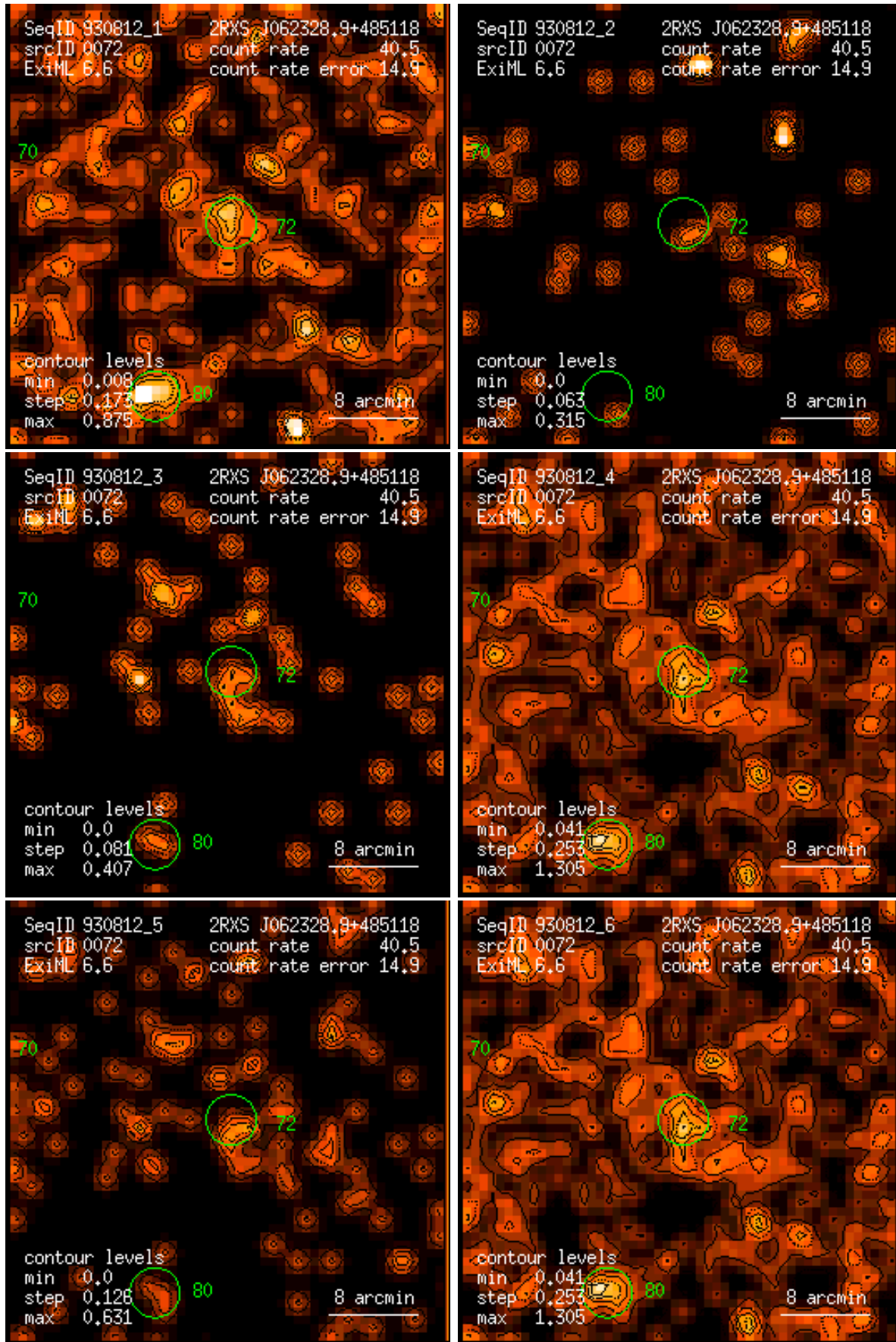
Figure 72: RASS 930812: detection 0072: band rate images, Gaussian filter: (1) PSPC channels 11 – 41, (2) 52 – 90, (3) 91 – 201, (4) 11 – 235, (5) 52 – 201, (6) 11 – 201. Broad band rates in counts/ks. Band rate contour levels in counts/ks/arcmin 2 .
