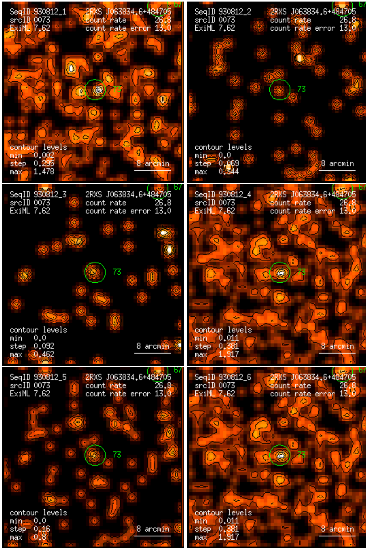
Figure 73: RASS 930812: detection 0073: band rate images, Gaussian filter: (1) PSPC channels 11 – 41, (2) 52 – 90, (3) 91 – 201, (4) 11 – 235, (5) 52 – 201, (6) 11 – 201. Broad band rates in counts/ks. Band rate contour levels in counts/ks/arcmin 2 .
