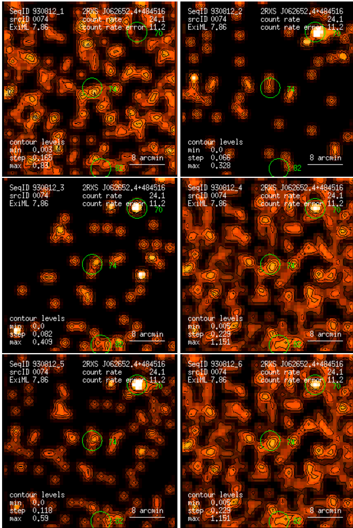
Figure 74: RASS 930812: detection 0074: band rate images, Gaussian filter: (1) PSPC channels 11 – 41, (2) 52 – 90, (3) 91 – 201, (4) 11 – 235, (5) 52 – 201, (6) 11 – 201. Broad band rates in counts/ks. Band rate contour levels in counts/ks/arcmin 2 .
