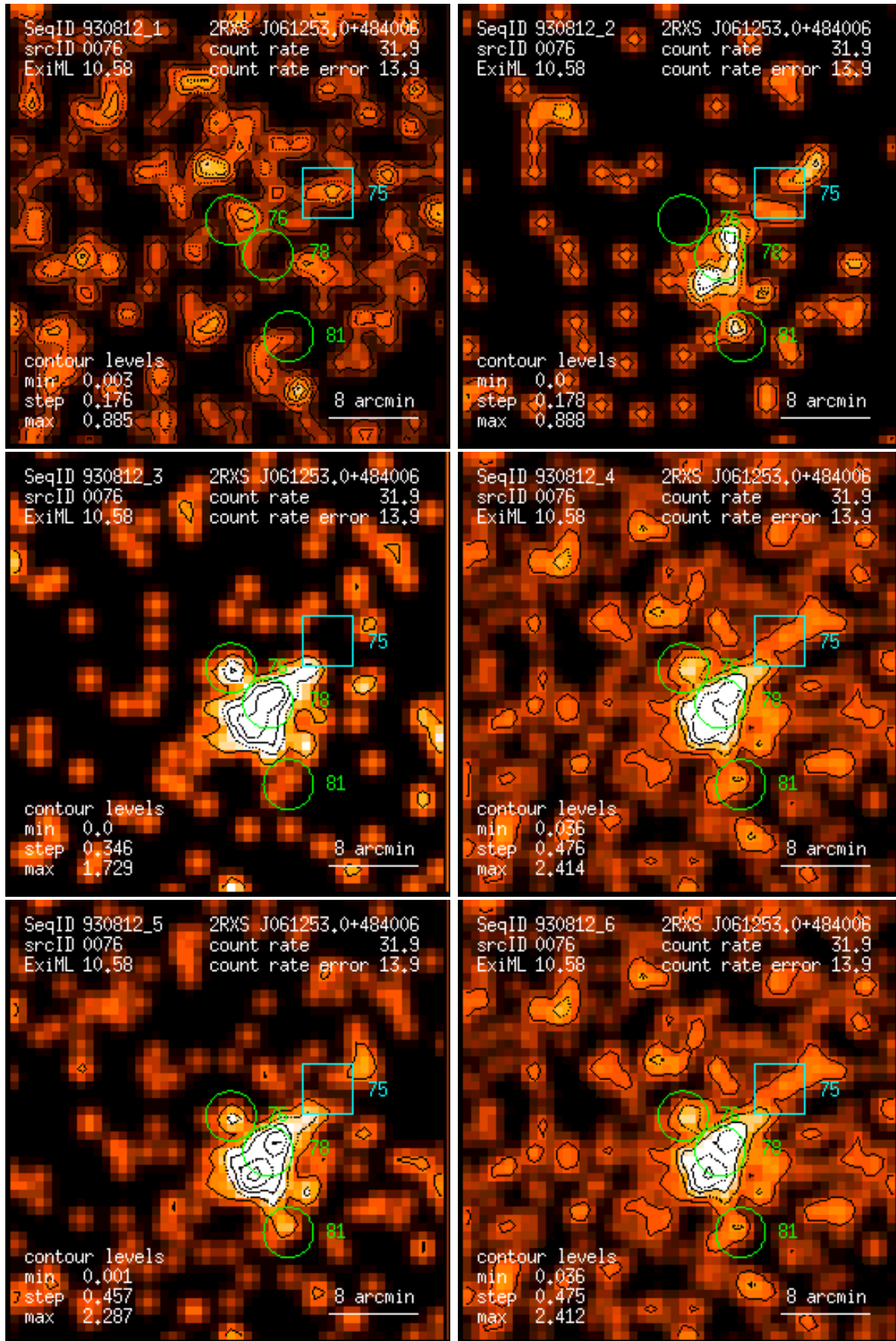
Figure 76: RASS 930812: detection 0076: band rate images, Gaussian filter: (1) PSPC channels 11 – 41, (2) 52 – 90, (3) 91 – 201, (4) 11 – 235, (5) 52 – 201, (6) 11 – 201. Broad band rates in counts/ks. Band rate contour levels in counts/ks/arcmin 2 .
