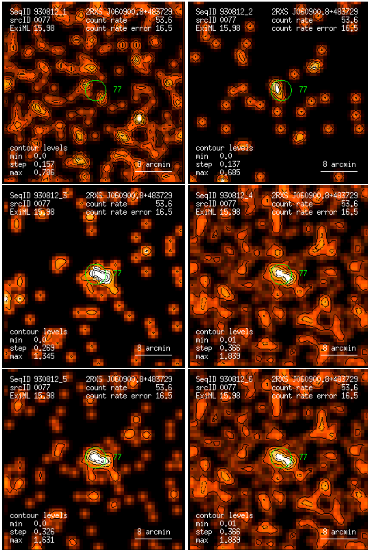
Figure 77: RASS 930812: detection 0077: band rate images, Gaussian filter: (1) PSPC channels 11 – 41, (2) 52 – 90, (3) 91 – 201, (4) 11 – 235, (5) 52 – 201, (6) 11 – 201. Broad band rates in counts/ks. Band rate contour levels in counts/ks/arcmin 2 .
