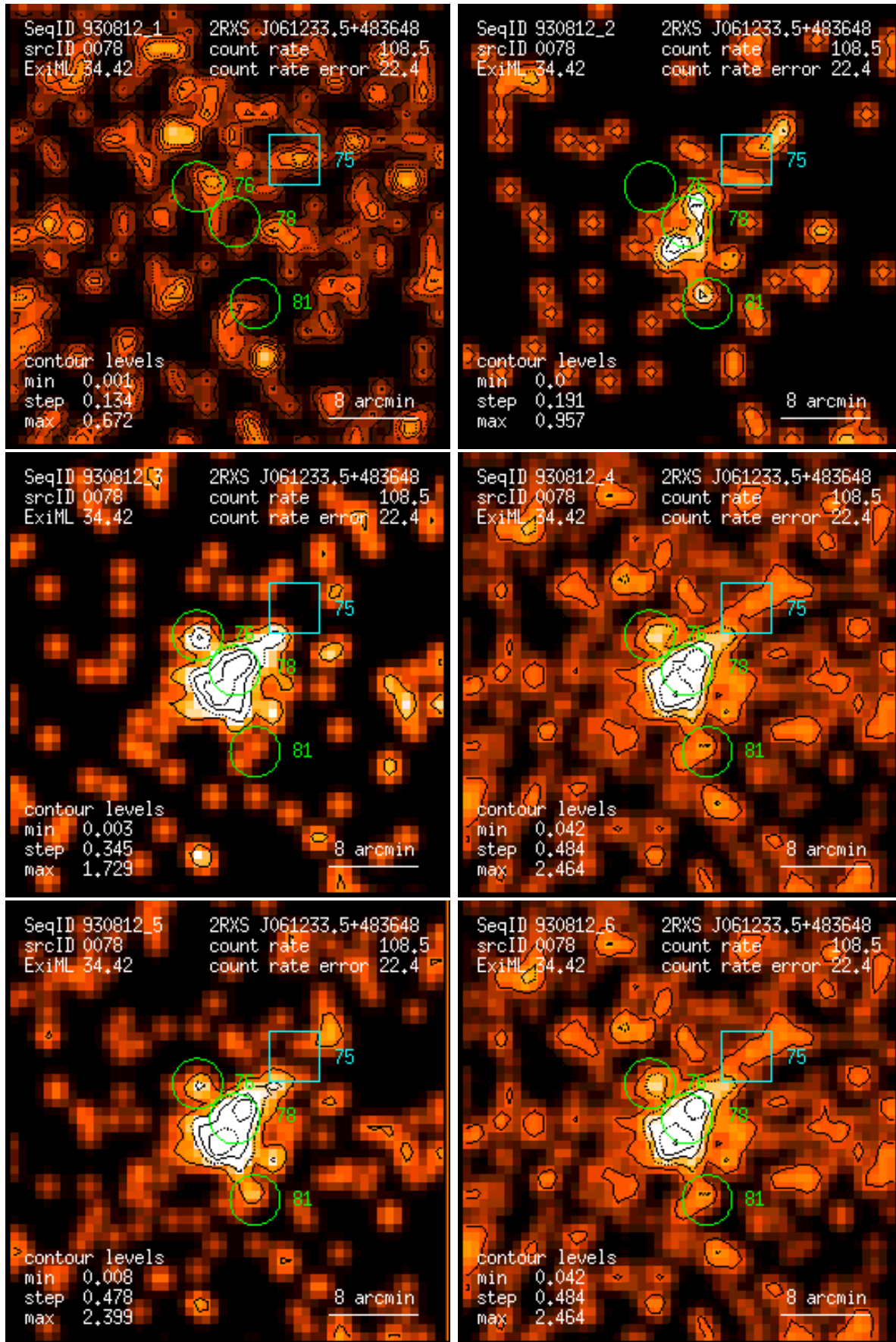
Figure 78: RASS 930812: detection 0078: band rate images, Gaussian filter: (1) PSPC channels 11 – 41, (2) 52 – 90, (3) 91 – 201, (4) 11 – 235, (5) 52 – 201, (6) 11 – 201. Broad band rates in counts/ks. Band rate contour levels in counts/ks/arcmin 2 .
