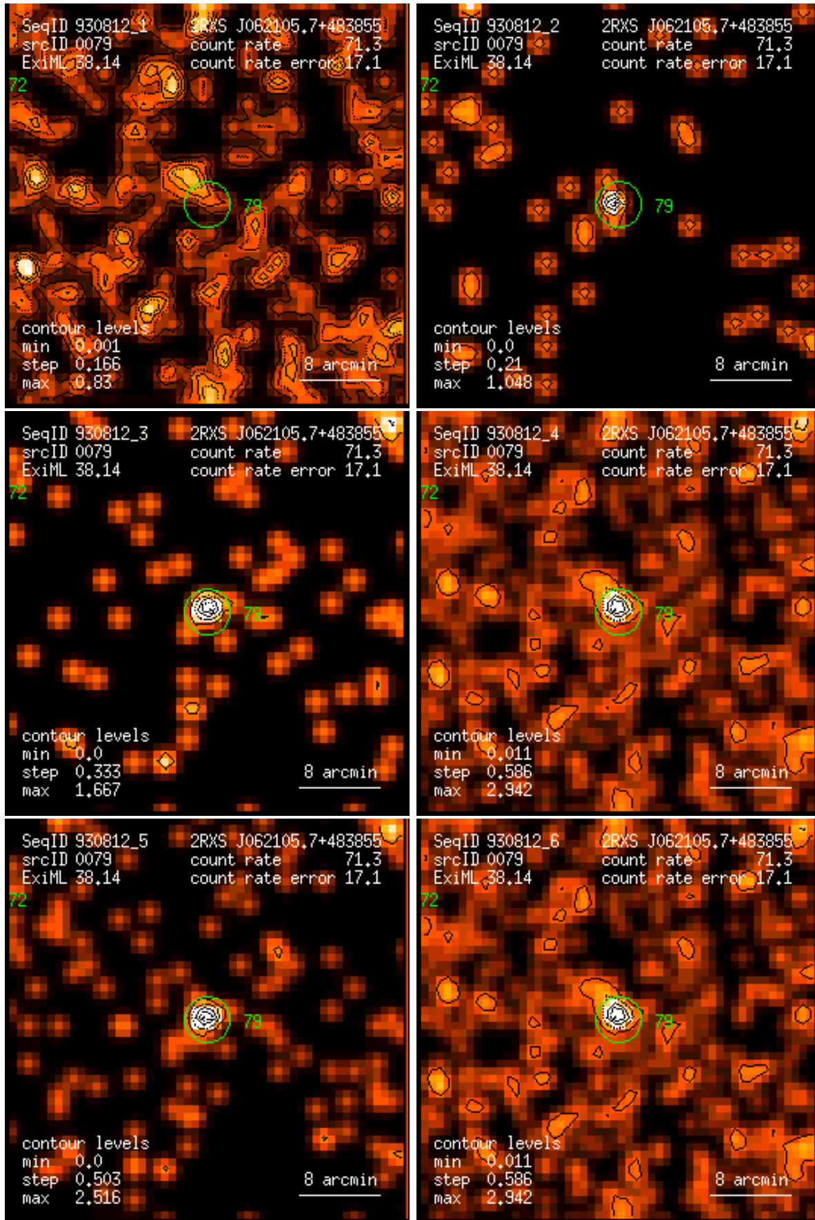
Figure 79: RASS 930812: detection 0079: band rate images, Gaussian filter: (1) PSPC channels 11 – 41, (2) 52 – 90, (3) 91 – 201, (4) 11 – 235, (5) 52 – 201, (6) 11 – 201. Broad band rates in counts/ks. Band rate contour levels in counts/ks/arcmin 2 .
