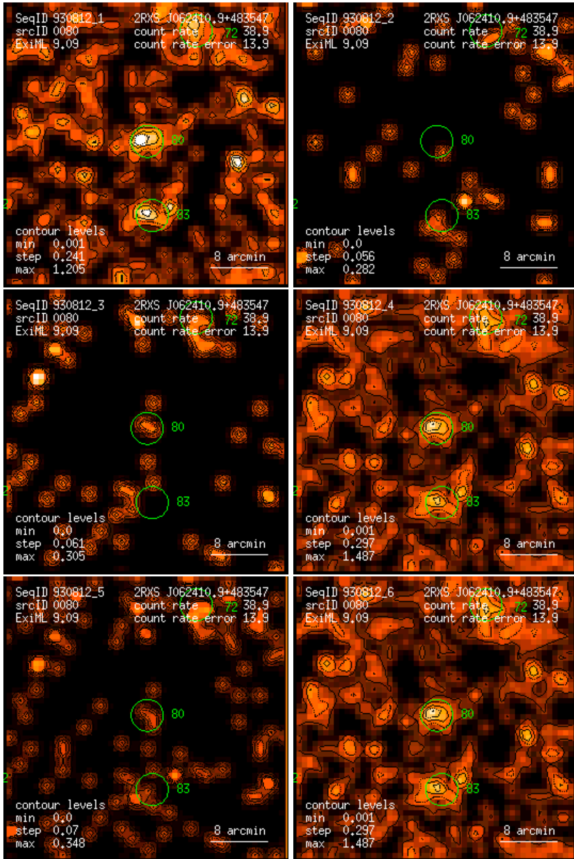
Figure 80: RASS 930812: detection 0080: band rate images, Gaussian filter: (1) PSPC channels 11 – 41, (2) 52 – 90, (3) 91 – 201, (4) 11 – 235, (5) 52 – 201, (6) 11 – 201. Broad band rates in counts/ks. Band rate contour levels in counts/ks/arcmin 2 .
