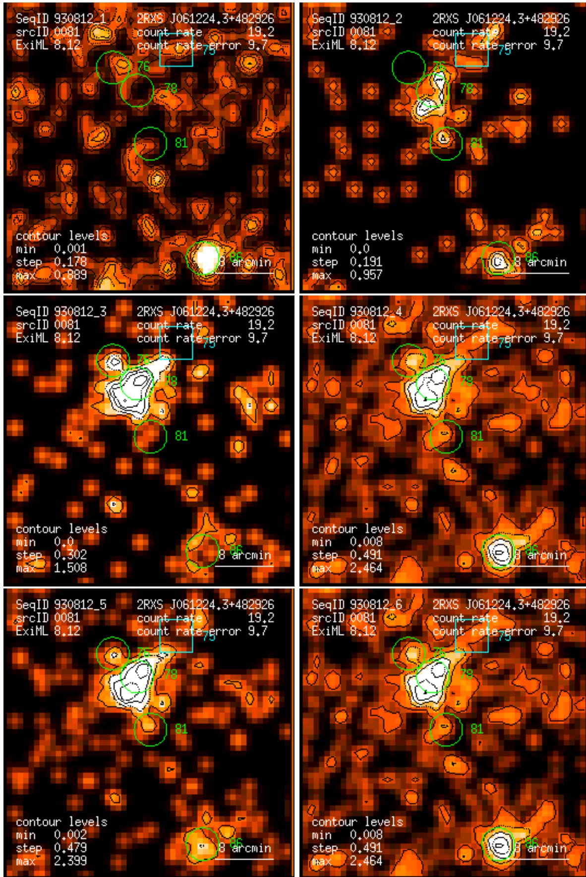
Figure 81: RASS 930812: detection 0081: band rate images, Gaussian filter: (1) PSPC channels 11 – 41, (2) 52 – 90, (3) 91 – 201, (4) 11 – 235, (5) 52 – 201, (6) 11 – 201. Broad band rates in counts/ks. Band rate contour levels in counts/ks/arcmin 2 .
