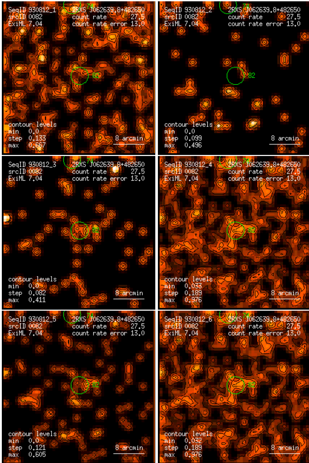
Figure 82: RASS 930812: detection 0082: band rate images, Gaussian filter: (1) PSPC channels 11 – 41, (2) 52 – 90, (3) 91 – 201, (4) 11 – 235, (5) 52 – 201, (6) 11 – 201. Broad band rates in counts/ks. Band rate contour levels in counts/ks/arcmin 2 .
