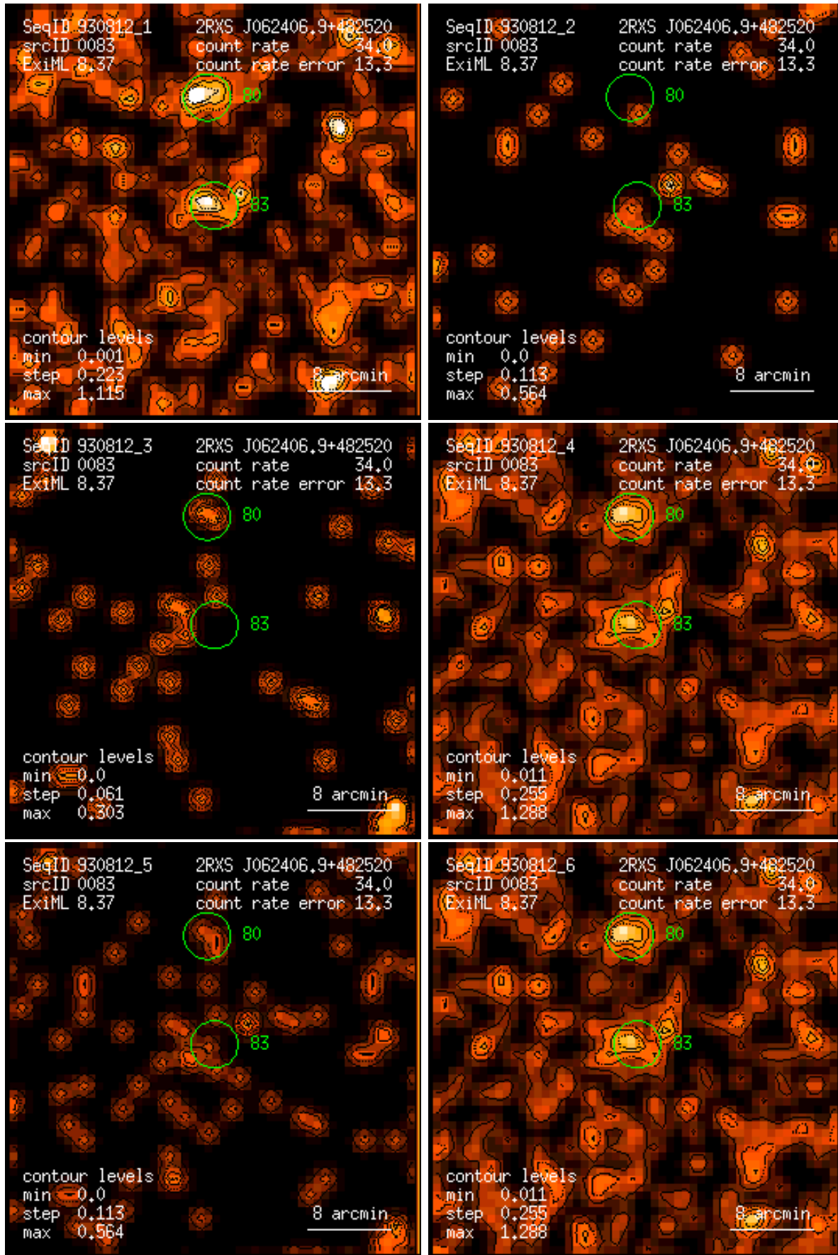
Figure 83: RASS 930812: detection 0083: band rate images, Gaussian filter: (1) PSPC channels 11 – 41, (2) 52 – 90, (3) 91 – 201, (4) 11 – 235, (5) 52 – 201, (6) 11 – 201. Broad band rates in counts/ks. Band rate contour levels in counts/ks/arcmin 2 .
