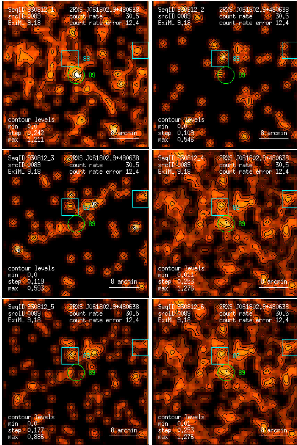
Figure 89: RASS 930812: detection 0089: band rate images, Gaussian filter: (1) PSPC channels 11 – 41, (2) 52 – 90, (3) 91 – 201, (4) 11 – 235, (5) 52 – 201, (6) 11 – 201. Broad band rates in counts/ks. Band rate contour levels in counts/ks/arcmin 2 .
