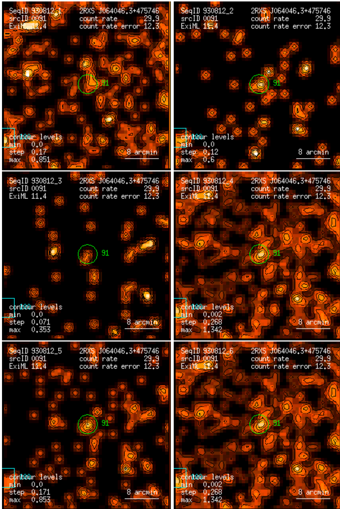
Figure 91: RASS 930812: detection 0091: band rate images, Gaussian filter: (1) PSPC channels 11 – 41, (2) 52 – 90, (3) 91 – 201, (4) 11 – 235, (5) 52 – 201, (6) 11 – 201. Broad band rates in counts/ks. Band rate contour levels in counts/ks/arcmin 2 .
