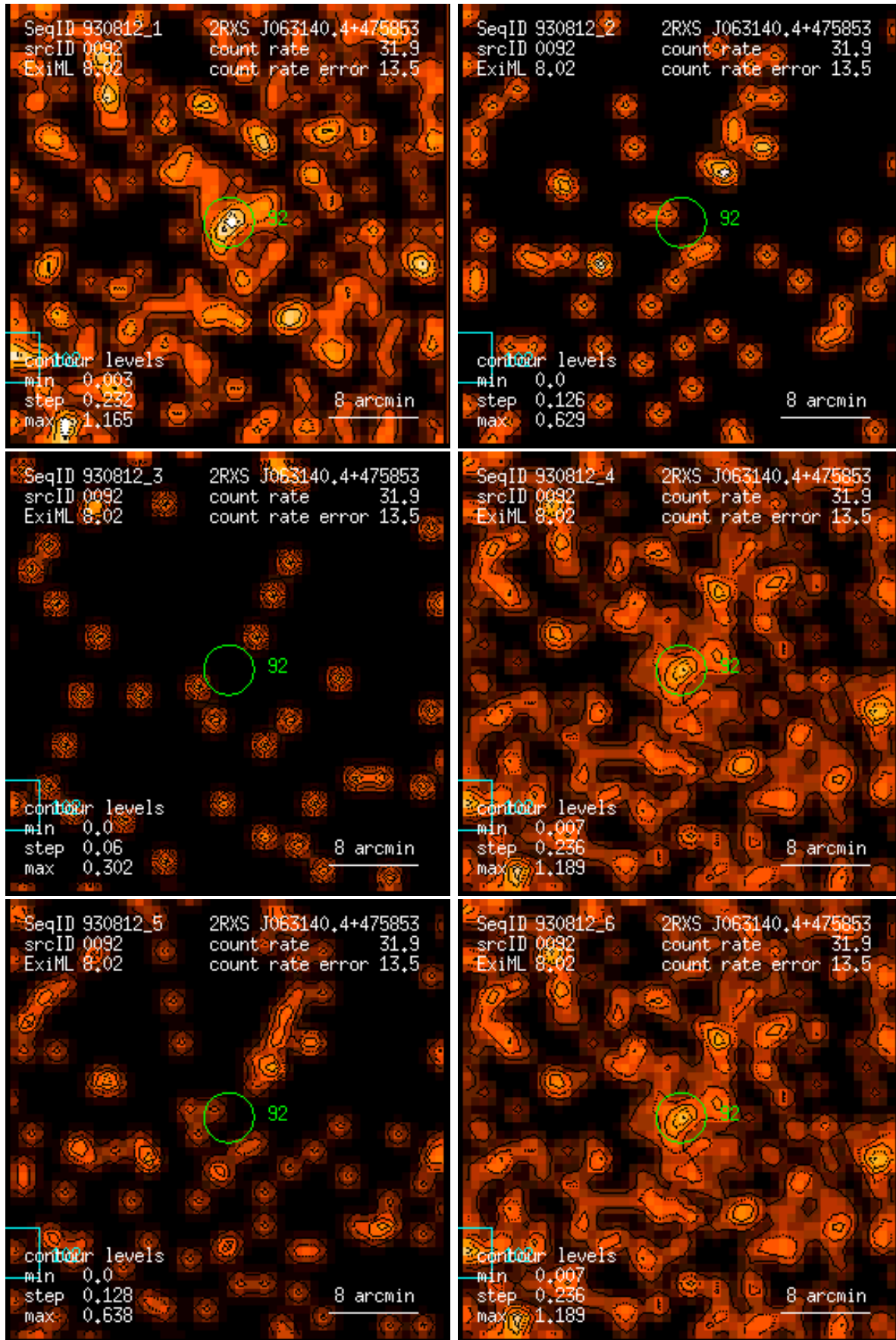
Figure 92: RASS 930812: detection 0092: band rate images, Gaussian filter: (1) PSPC channels 11 – 41, (2) 52 – 90, (3) 91 – 201, (4) 11 – 235, (5) 52 – 201, (6) 11 – 201. Broad band rates in counts/ks. Band rate contour levels in counts/ks/arcmin 2 .
