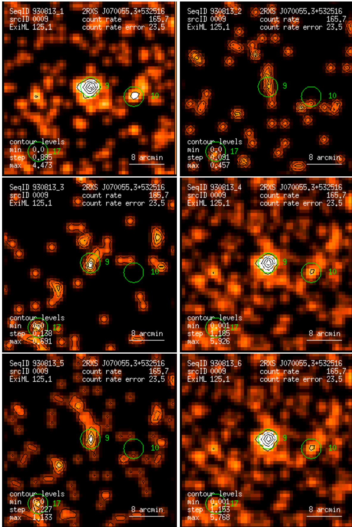
Figure 9: RASS 930813: detection 0009: band rate images, Gaussian filter: (1) PSPC channels 11 – 41, (2) 52 – 90, (3) 91 – 201, (4) 11 – 235, (5) 52 – 201, (6) 11 – 201. Broad band rates in counts/ks. Band rate contour levels in counts/ks/arcmin 2 .
