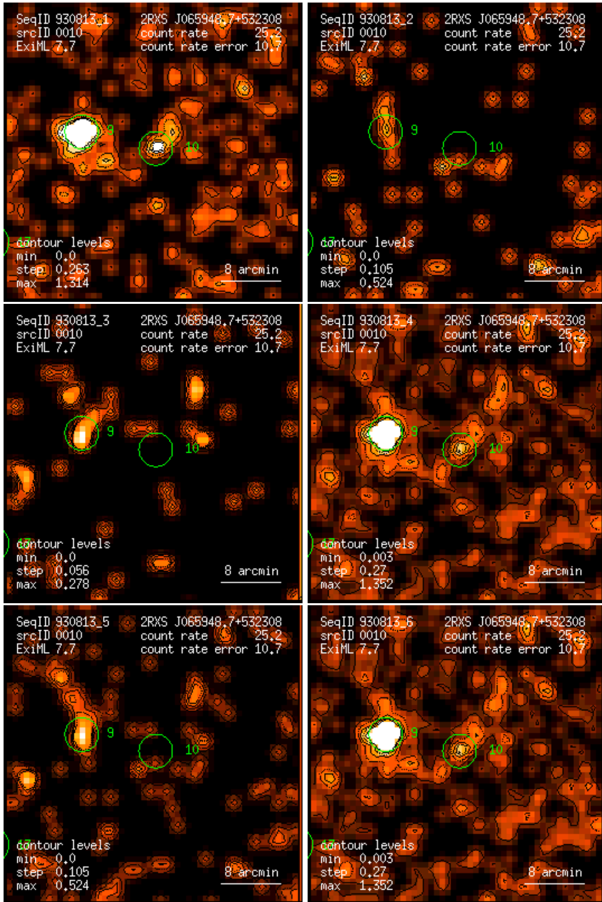
Figure 10: RASS 930813: detection 0010: band rate images, Gaussian filter: (1) PSPC channels 11 – 41, (2) 52 – 90, (3) 91 – 201, (4) 11 – 235, (5) 52 – 201, (6) 11 – 201. Broad band rates in counts/ks. Band rate contour levels in counts/ks/arcmin 2 .
