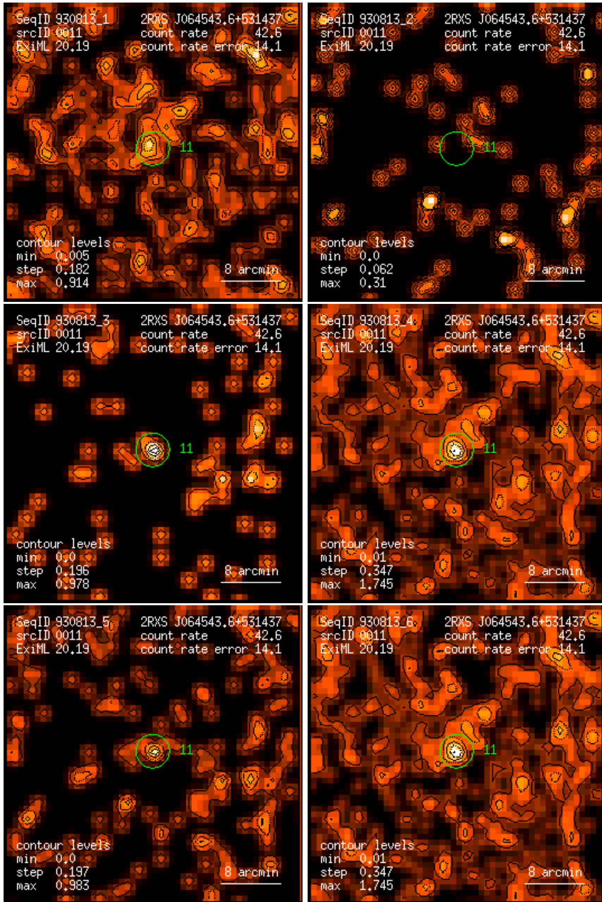
Figure 11: RASS 930813: detection 0011: band rate images, Gaussian filter: (1) PSPC channels 11 – 41, (2) 52 – 90, (3) 91 – 201, (4) 11 – 235, (5) 52 – 201, (6) 11 – 201. Broad band rates in counts/ks. Band rate contour levels in counts/ks/arcmin 2 .
