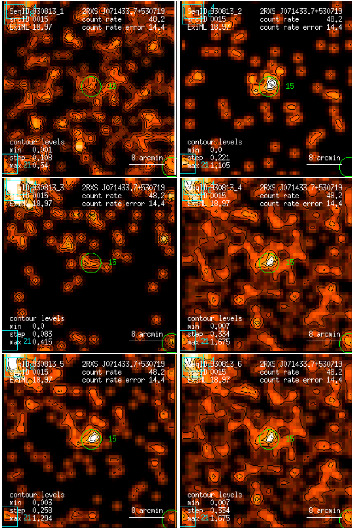
Figure 15: RASS 930813: detection 0015: band rate images, Gaussian filter: (1) PSPC channels 11 – 41, (2) 52 – 90, (3) 91 – 201, (4) 11 – 235, (5) 52 – 201, (6) 11 – 201. Broad band rates in counts/ks. Band rate contour levels in counts/ks/arcmin 2 .
