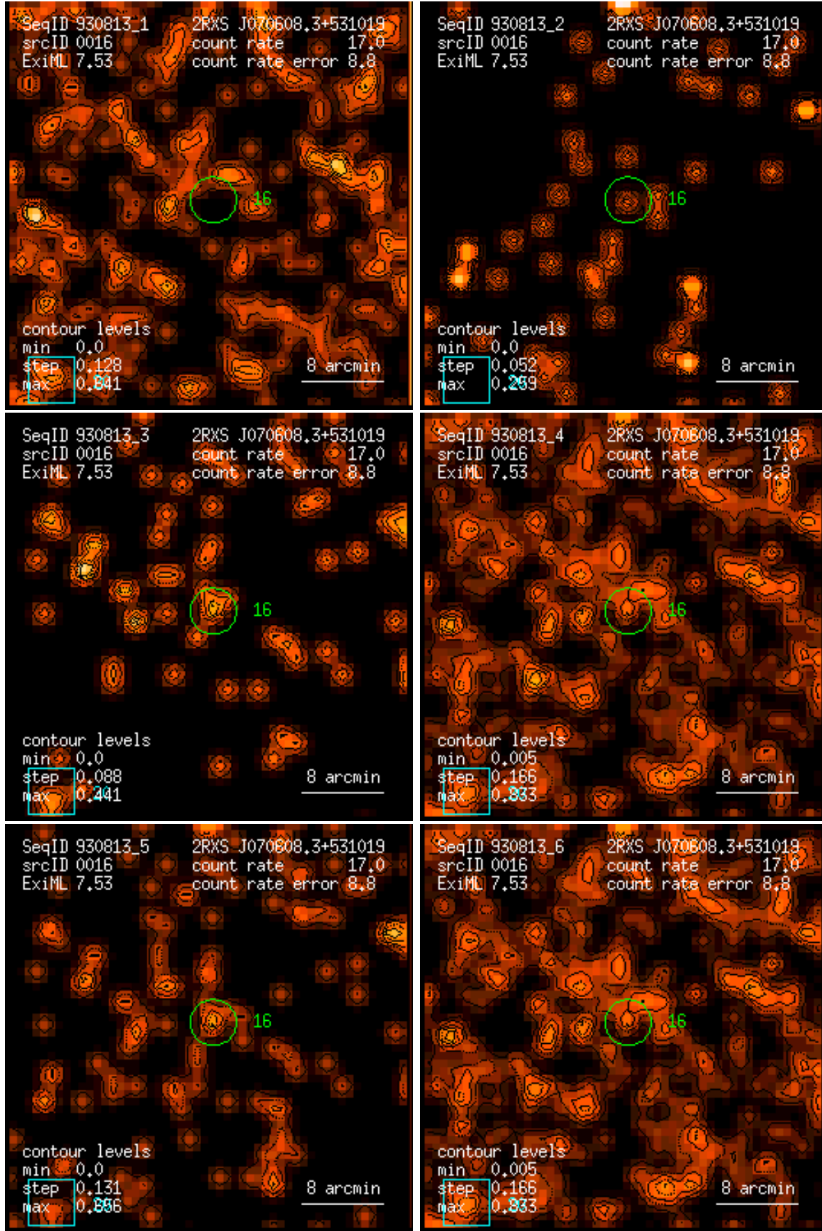
Figure 16: RASS 930813: detection 0016: band rate images, Gaussian filter: (1) PSPC channels 11 – 41, (2) 52 – 90, (3) 91 – 201, (4) 11 – 235, (5) 52 – 201, (6) 11 – 201. Broad band rates in counts/ks. Band rate contour levels in counts/ks/arcmin 2 .
