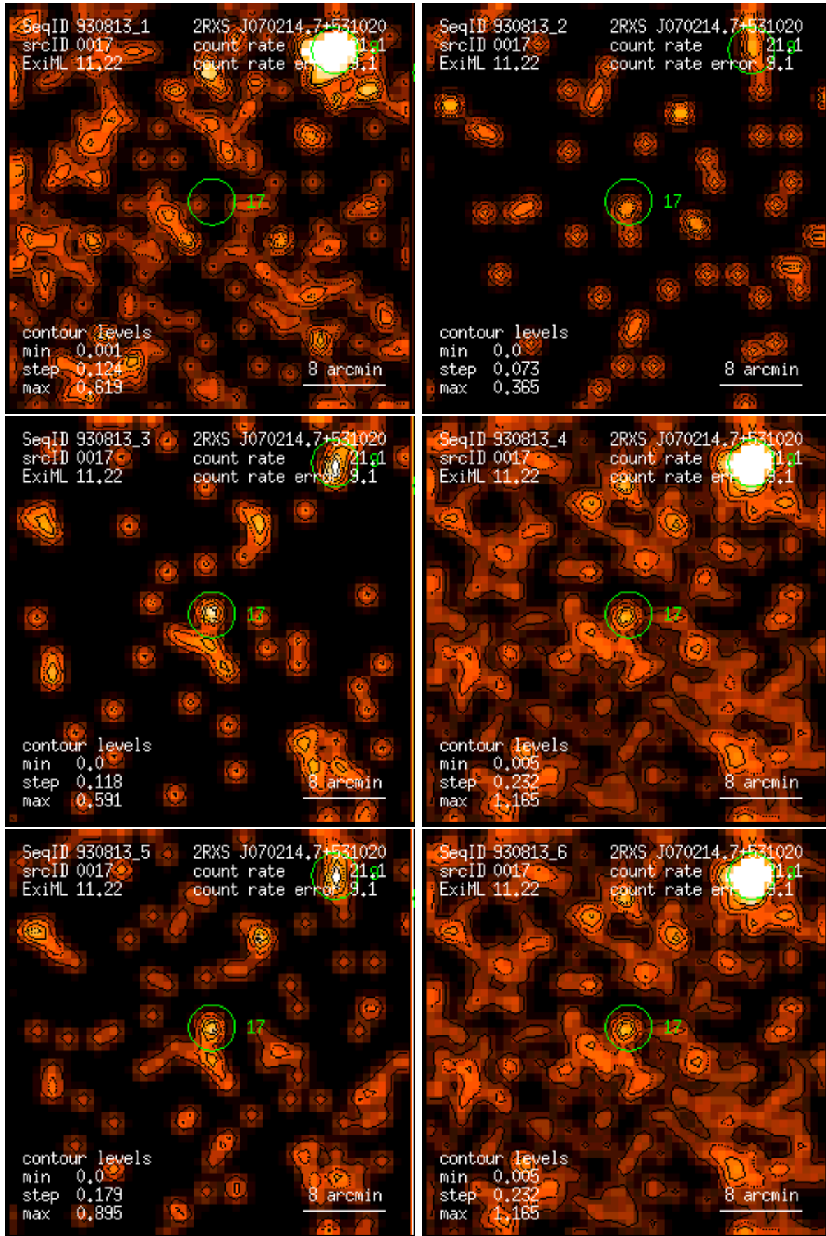
Figure 17: RASS 930813: detection 0017: band rate images, Gaussian filter: (1) PSPC channels 11 – 41, (2) 52 – 90, (3) 91 – 201, (4) 11 – 235, (5) 52 – 201, (6) 11 – 201. Broad band rates in counts/ks. Band rate contour levels in counts/ks/arcmin 2 .
