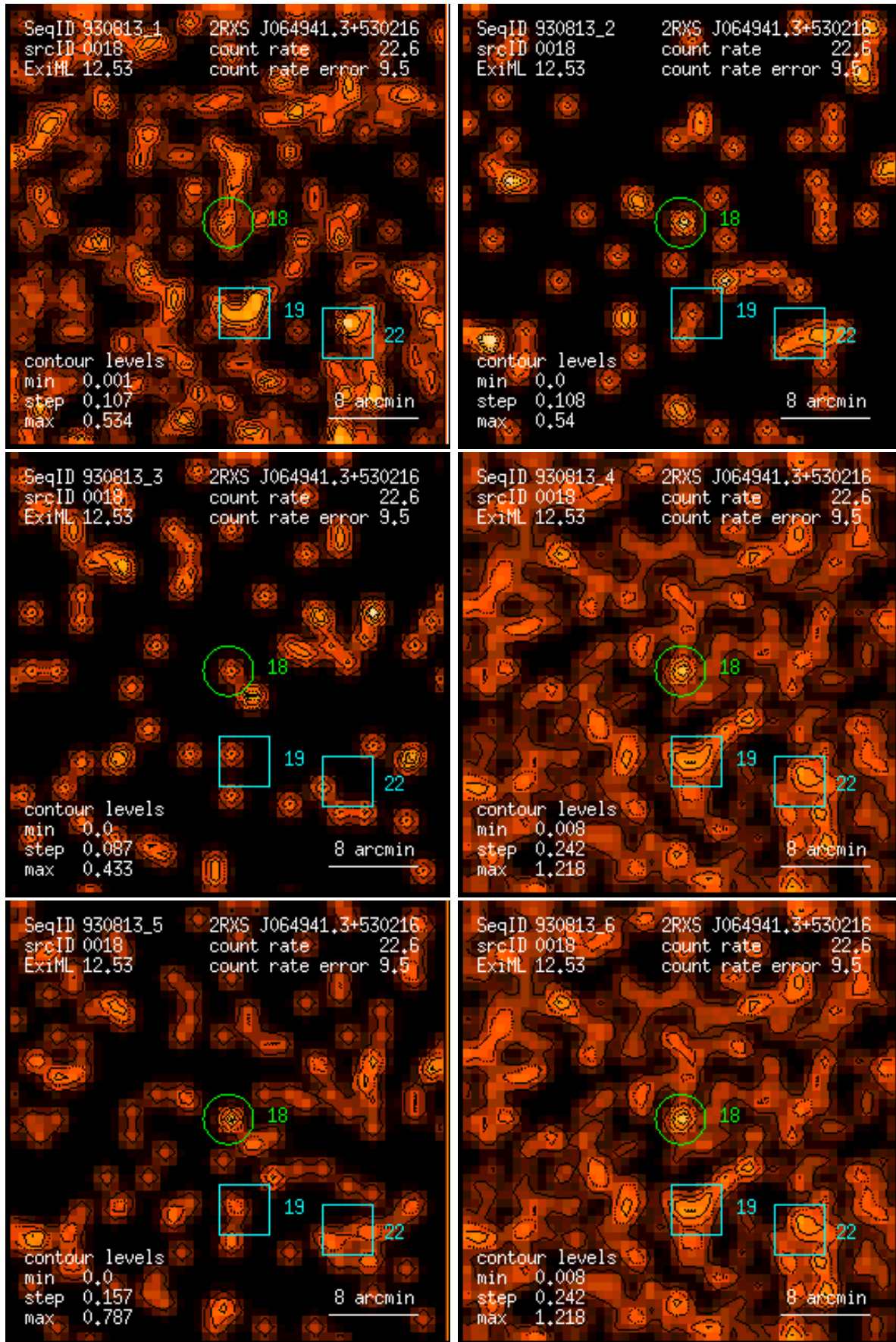
Figure 18: RASS 930813: detection 0018: band rate images, Gaussian filter: (1) PSPC channels 11 – 41, (2) 52 – 90, (3) 91 – 201, (4) 11 – 235, (5) 52 – 201, (6) 11 – 201. Broad band rates in counts/ks. Band rate contour levels in counts/ks/arcmin 2 .
