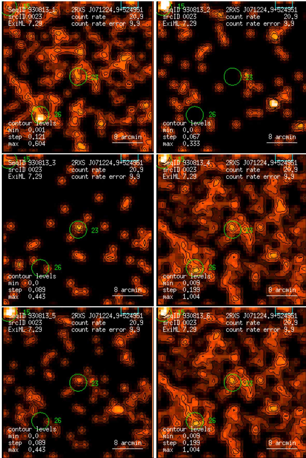
Figure 23: RASS 930813: detection 0023: band rate images, Gaussian filter: (1) PSPC channels 11 – 41, (2) 52 – 90, (3) 91 – 201, (4) 11 – 235, (5) 52 – 201, (6) 11 – 201. Broad band rates in counts/ks. Band rate contour levels in counts/ks/arcmin 2 .
