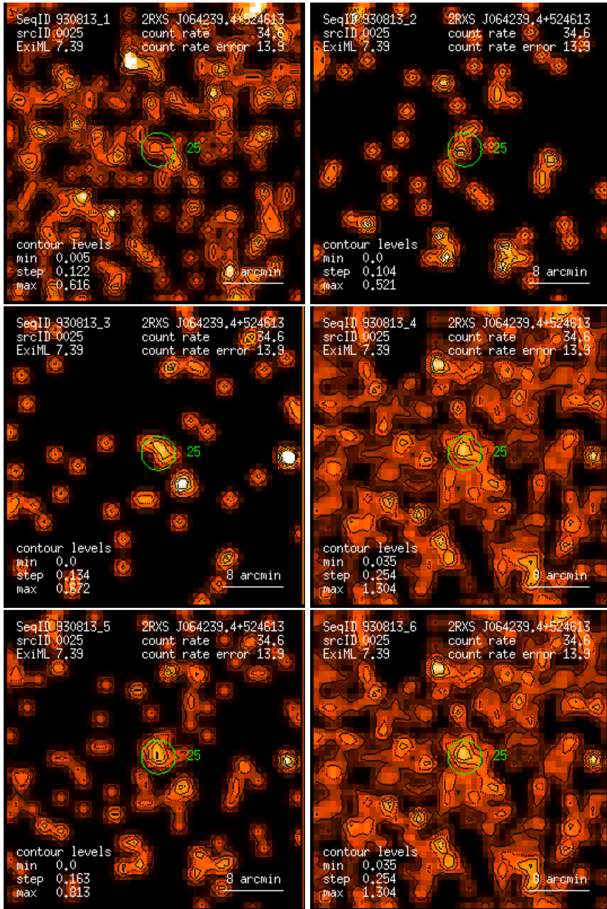
Figure 25: RASS 930813: detection 0025: band rate images, Gaussian filter: (1) PSPC channels 11 – 41, (2) 52 – 90, (3) 91 – 201, (4) 11 – 235, (5) 52 – 201, (6) 11 – 201. Broad band rates in counts/ks. Band rate contour levels in counts/ks/arcmin 2 .
