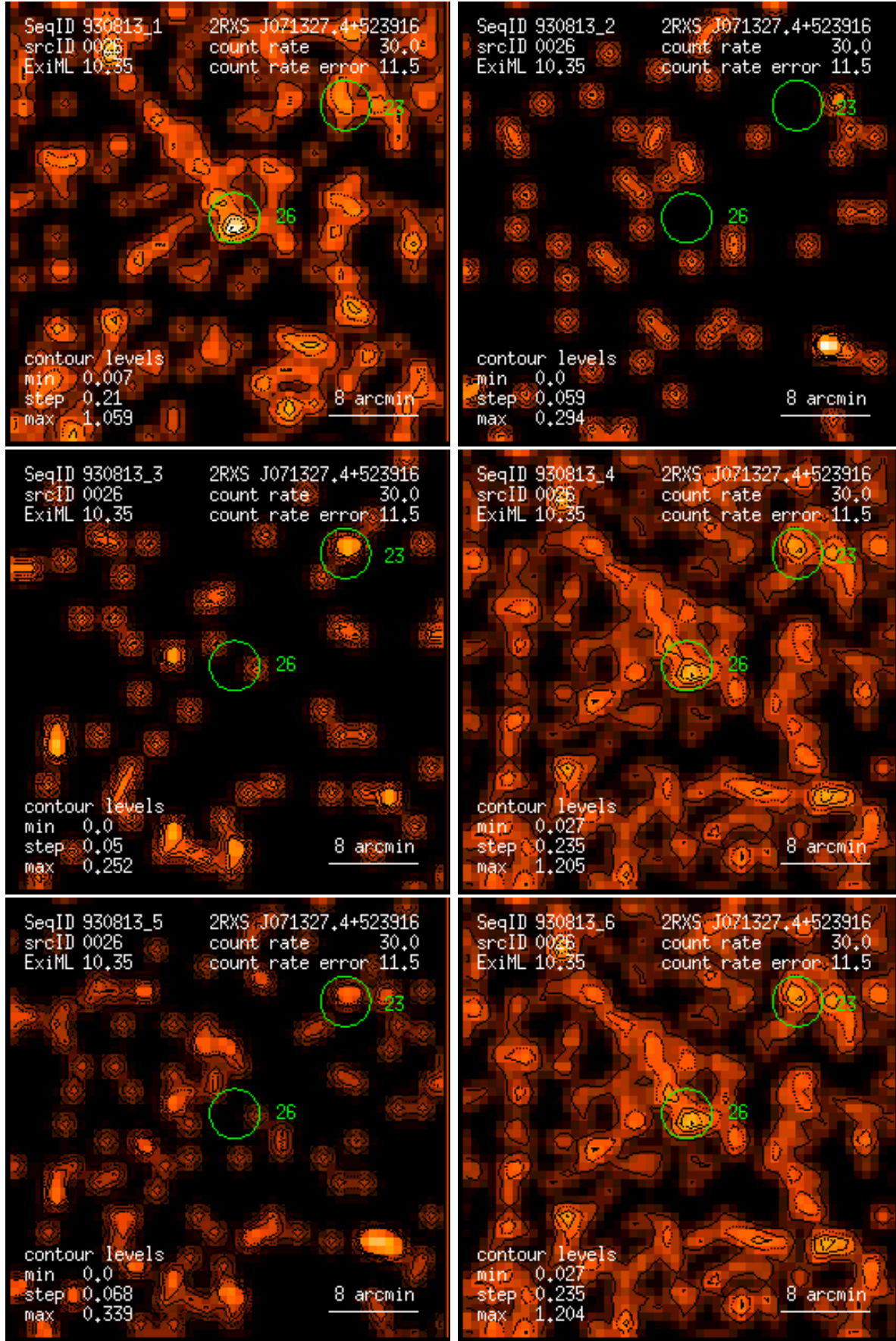
Figure 26: RASS 930813: detection 0026: band rate images, Gaussian filter: (1) PSPC channels 11 – 41, (2) 52 – 90, (3) 91 – 201, (4) 11 – 235, (5) 52 – 201, (6) 11 – 201. Broad band rates in counts/ks. Band rate contour levels in counts/ks/arcmin 2 .
