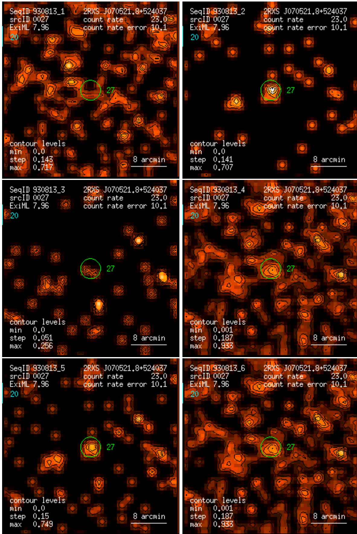
Figure 27: RASS 930813: detection 0027: band rate images, Gaussian filter: (1) PSPC channels 11 – 41, (2) 52 – 90, (3) 91 – 201, (4) 11 – 235, (5) 52 – 201, (6) 11 – 201. Broad band rates in counts/ks. Band rate contour levels in counts/ks/arcmin 2 .
