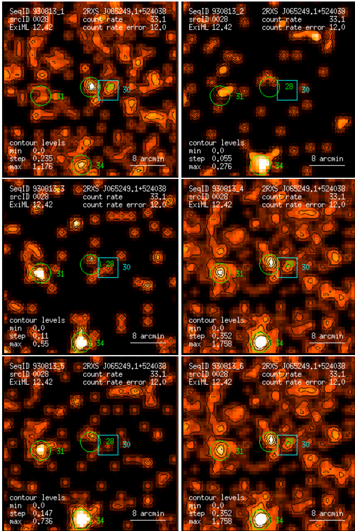
Figure 28: RASS 930813: detection 0028: band rate images, Gaussian filter: (1) PSPC channels 11 – 41, (2) 52 – 90, (3) 91 – 201, (4) 11 – 235, (5) 52 – 201, (6) 11 – 201. Broad band rates in counts/ks. Band rate contour levels in counts/ks/arcmin 2 .
