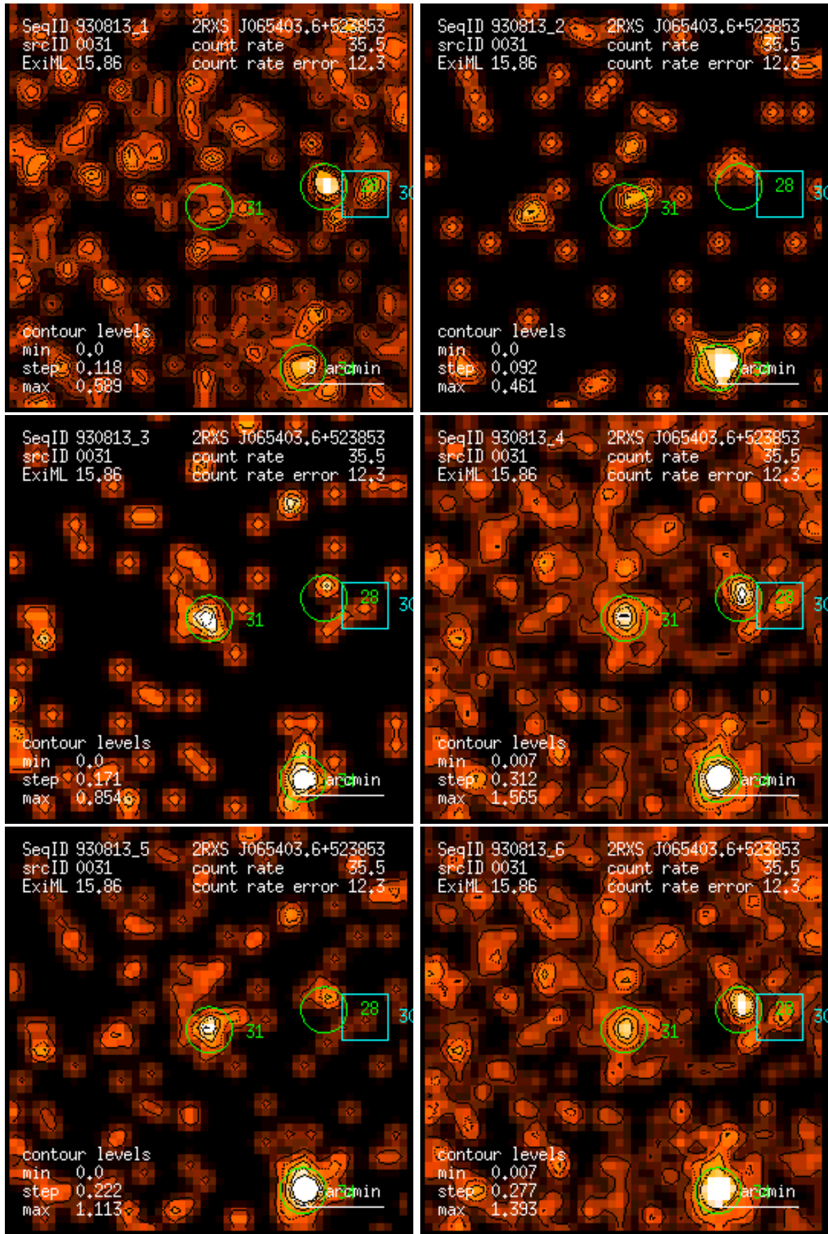
Figure 31: RASS 930813: detection 0031: band rate images, Gaussian filter: (1) PSPC channels 11 – 41, (2) 52 – 90, (3) 91 – 201, (4) 11 – 235, (5) 52 – 201, (6) 11 – 201. Broad band rates in counts/ks. Band rate contour levels in counts/ks/arcmin 2 .
