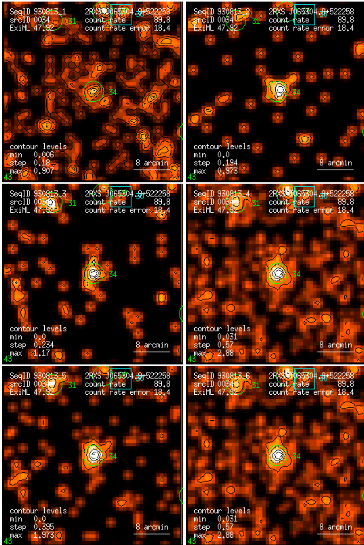
Figure 34: RASS 930813: detection 0034: band rate images, Gaussian filter: (1) PSPC channels 11 – 41, (2) 52 – 90, (3) 91 – 201, (4) 11 – 235, (5) 52 – 201, (6) 11 – 201. Broad band rates in counts/ks. Band rate contour levels in counts/ks/arcmin 2 .
