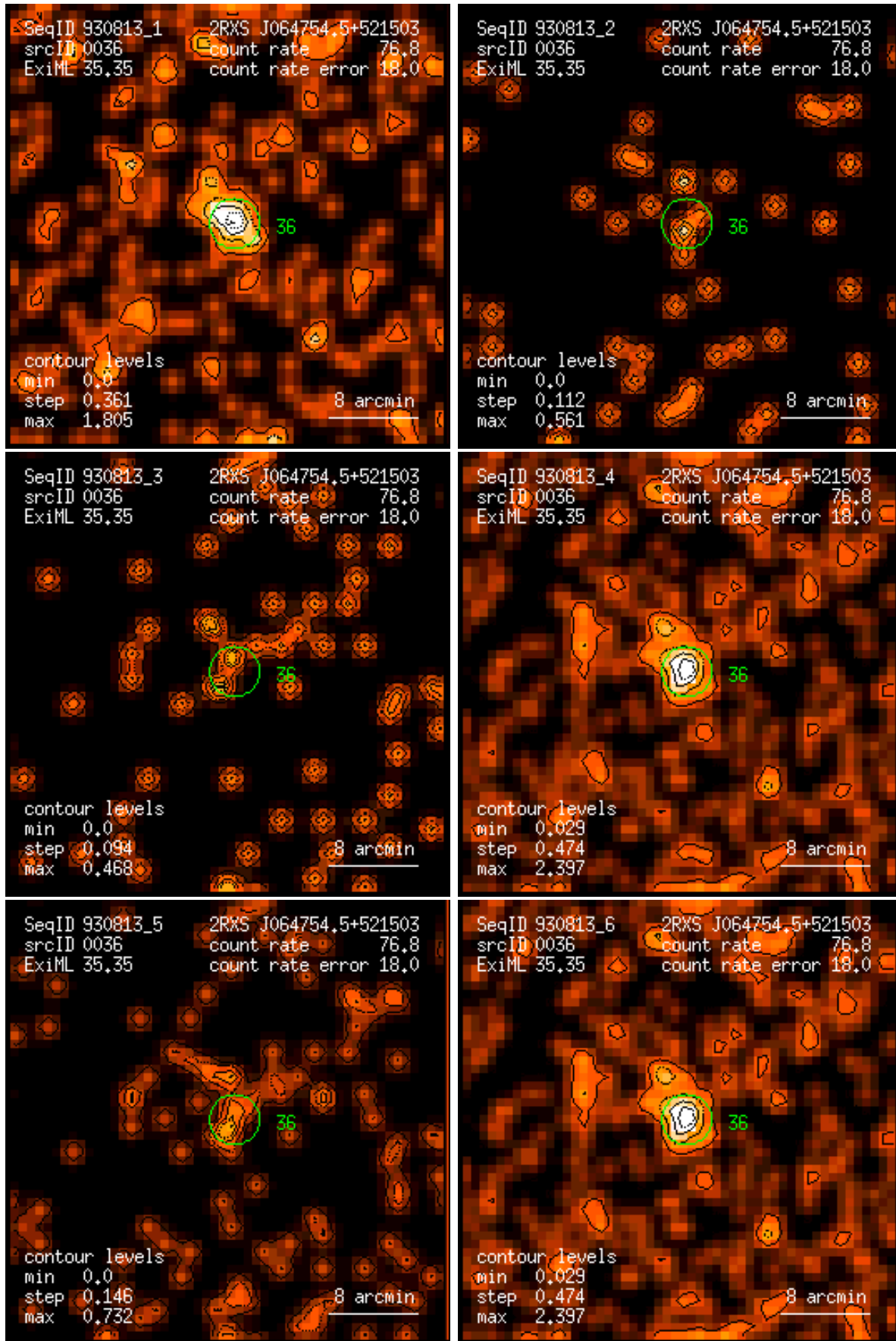
Figure 36: RASS 930813: detection 0036: band rate images, Gaussian filter: (1) PSPC channels 11 – 41, (2) 52 – 90, (3) 91 – 201, (4) 11 – 235, (5) 52 – 201, (6) 11 – 201. Broad band rates in counts/ks. Band rate contour levels in counts/ks/arcmin 2 .
